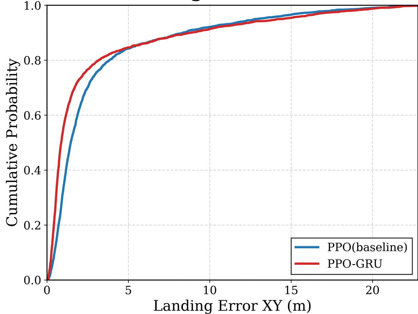
DRDP Precision CDF: PPO(baseline) vs PPO-GRU Landing Error XY CDF
