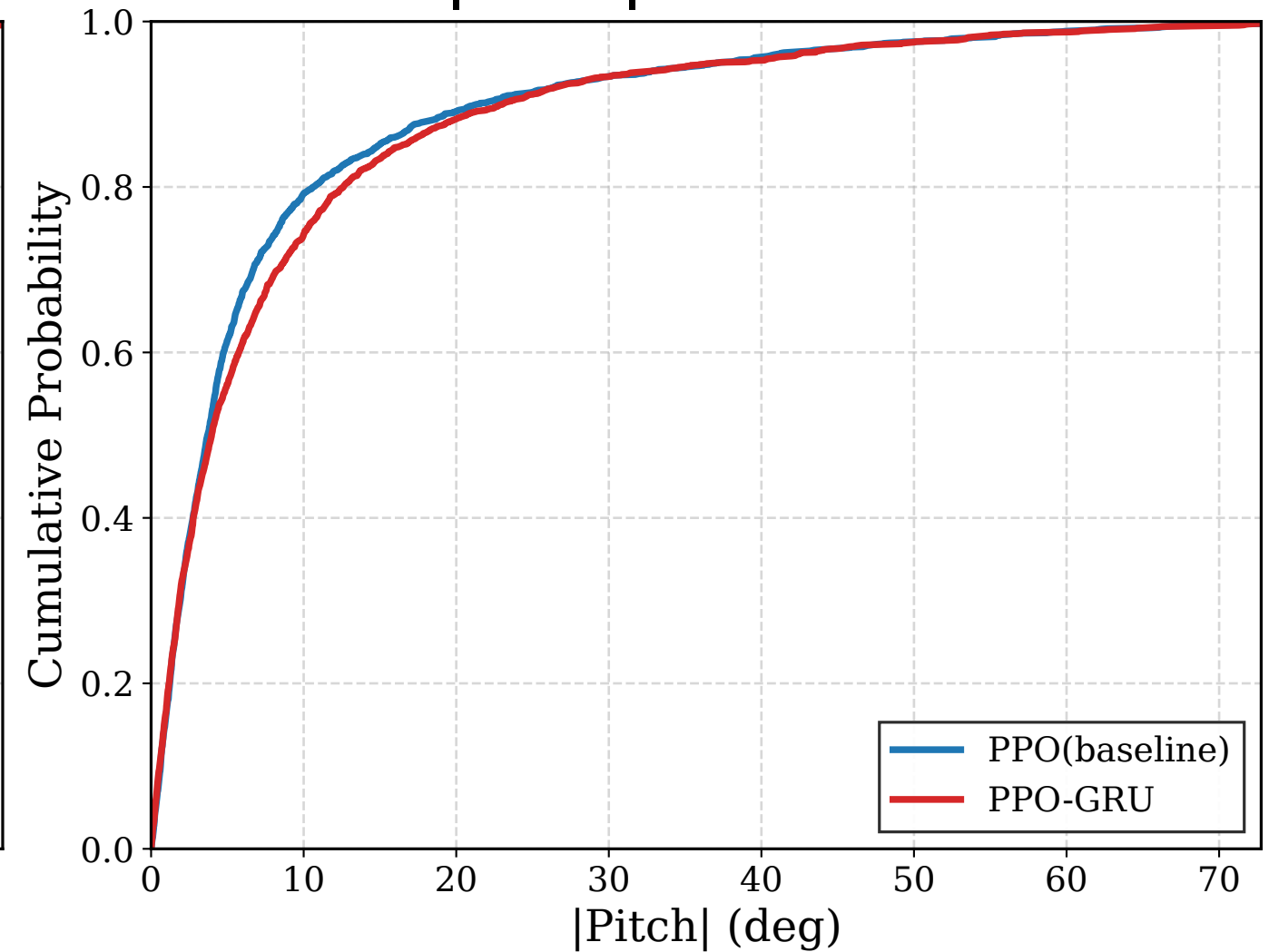
|Pitch| Error CDF
