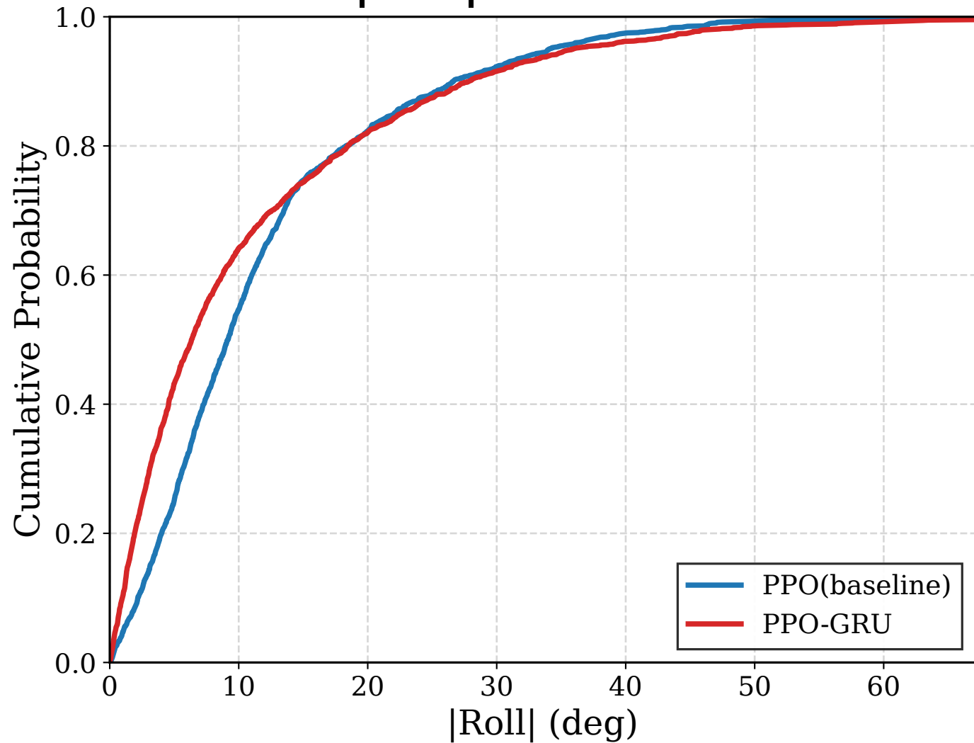
|Roll| Error CDF
