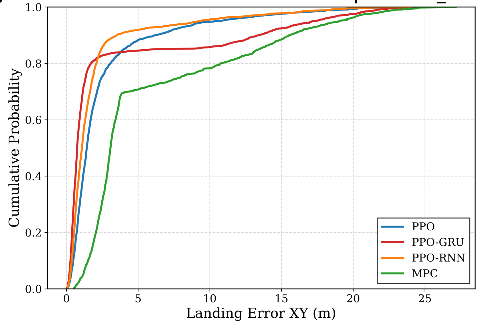
Experiment 2: Fixed Height + Fixed Wind + Obstacle Ablation | random_obstacle | Landing Precision CDF
