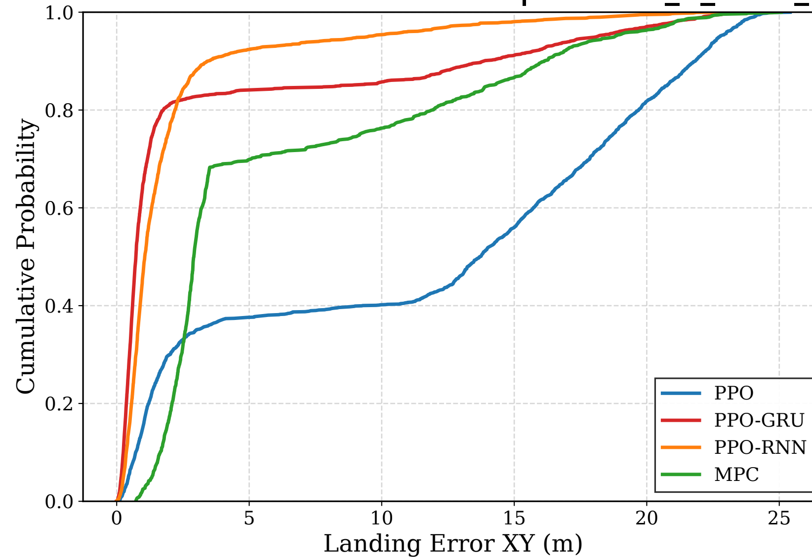
Experiment 3: Random Height + Fixed Wind + Fixed Obstacle | random_h_fixed_w_fixed_obs | Landing Precision CDF
