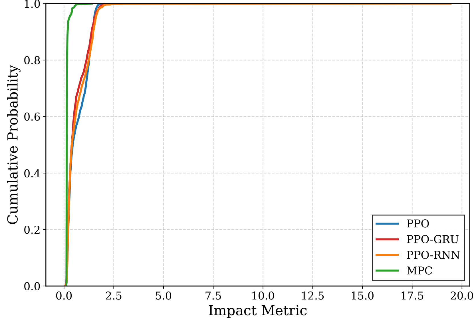
Experiment 4: Fixed Height + Obstacle + Multi Wind Strength | strong_wind | Impact CDF
