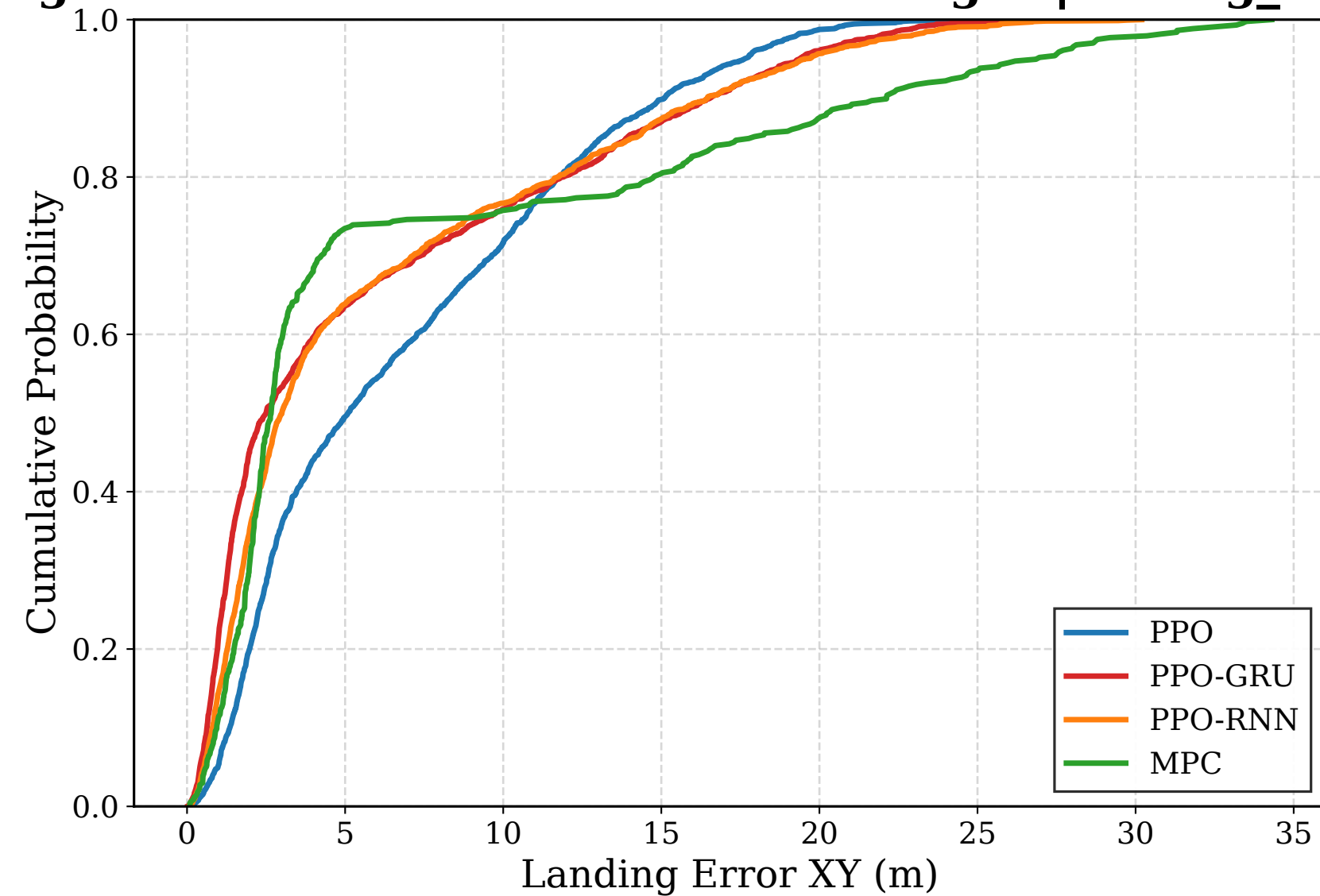
Experiment 4: Fixed Height + Obstacle + Multi Wind Strength | strong_wind | Landing Precision CDF
