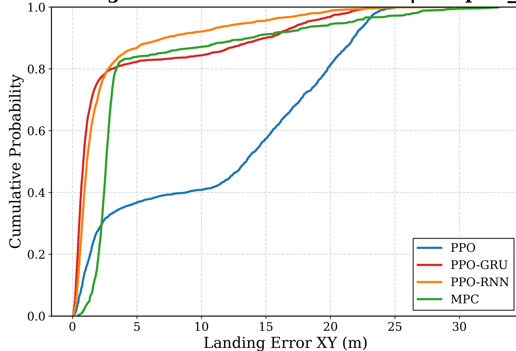
Experiment 5: Complex Multi-Height + Multi-Wind + Obstacle | complex_mix | Landing Precision CDF
