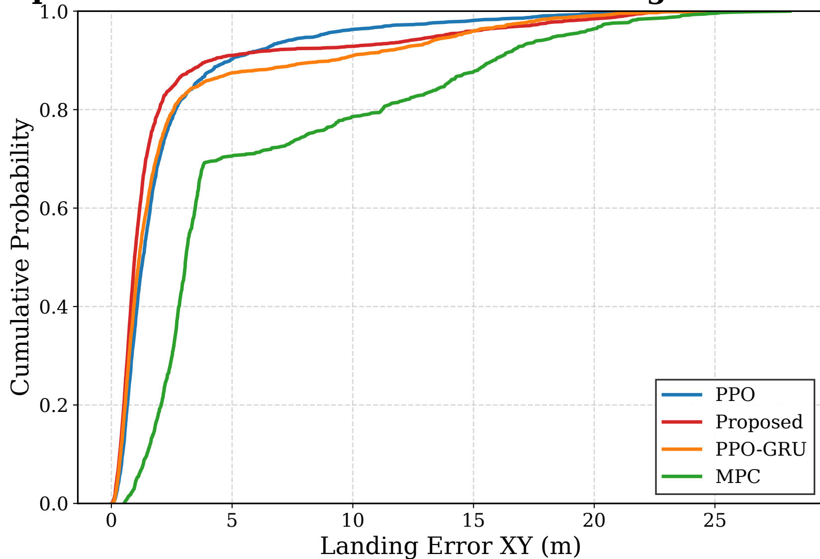
Experiment 2-Random Obstacle: Landing Precision CDF
