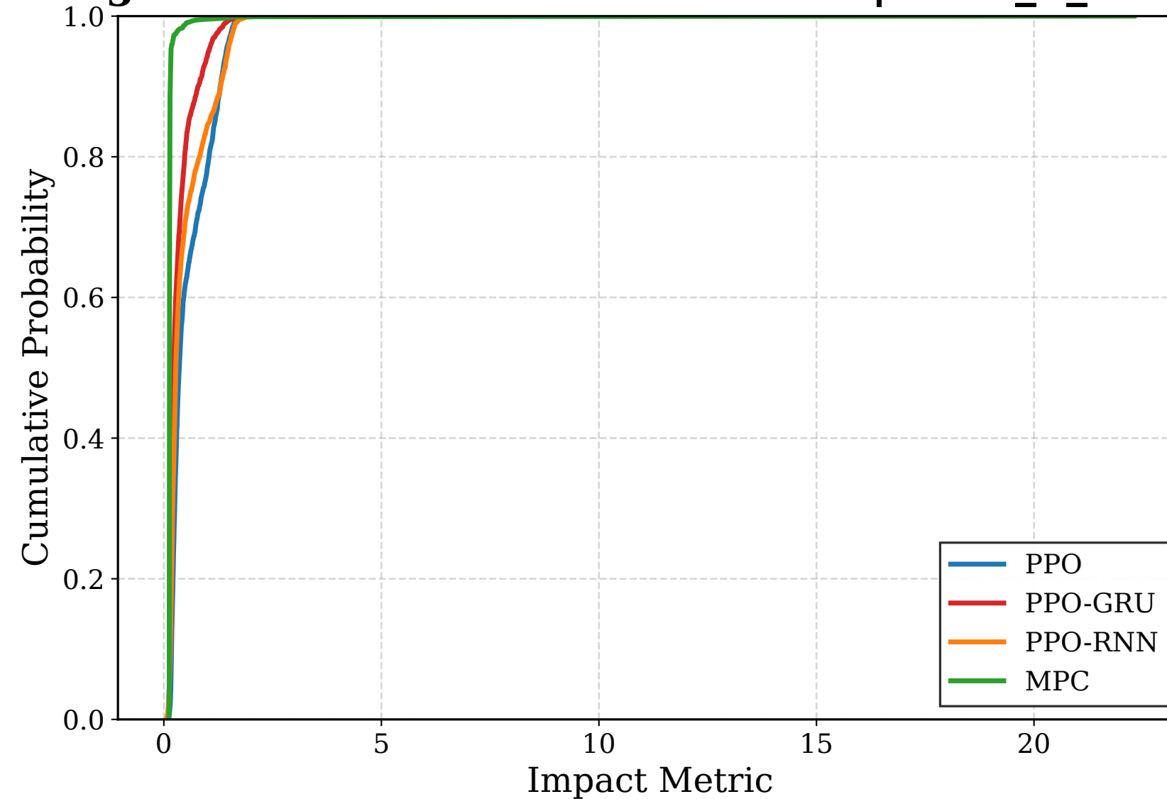
Experiment 1: Fixed Height + Fixed Wind + No Obstacle | fixed_h_fixed_w_no_obs | Impact CDF
