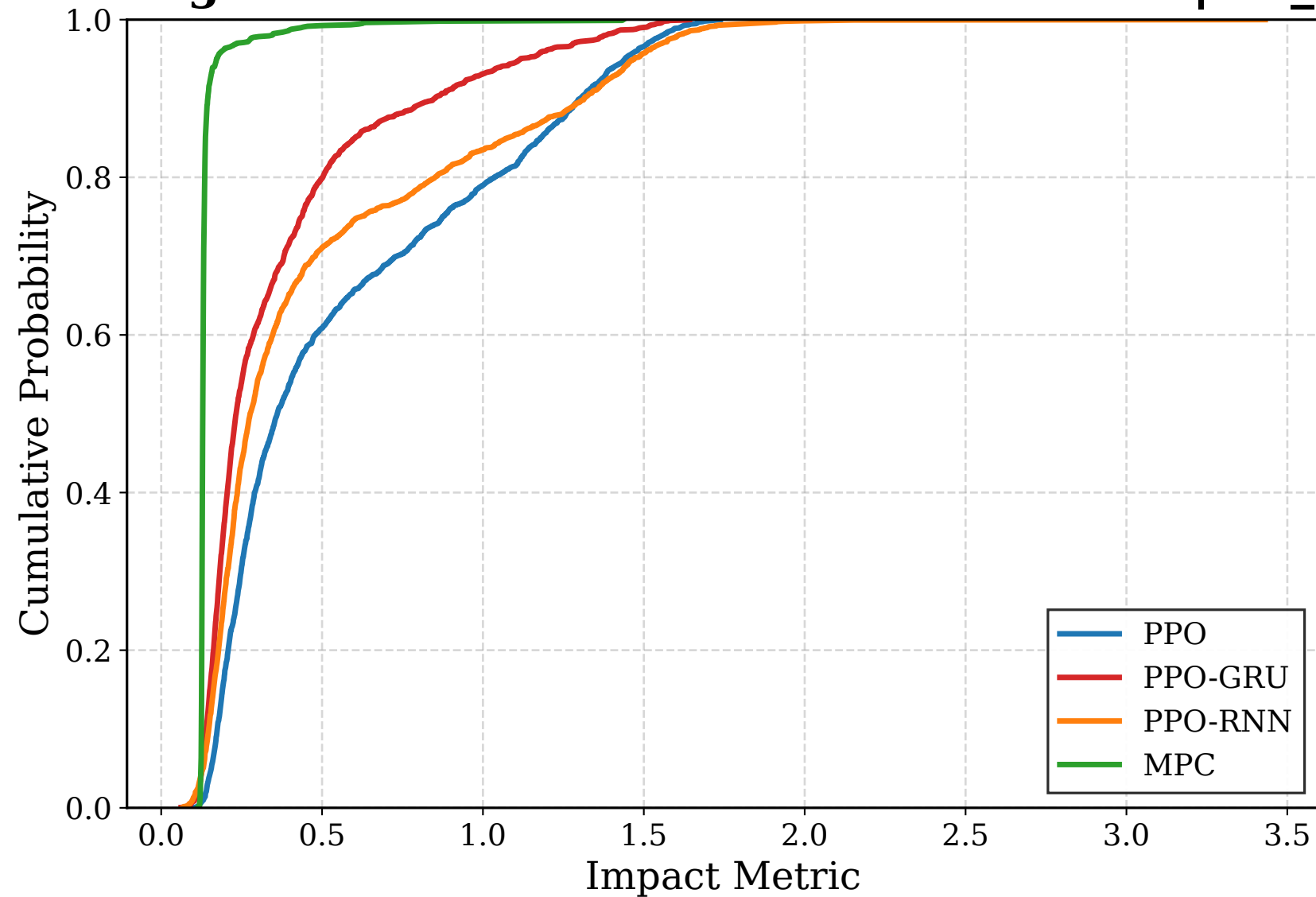
Experiment 2: Fixed Height + Fixed Wind + Obstacle Ablation | no_obstacle | Impact CDF
