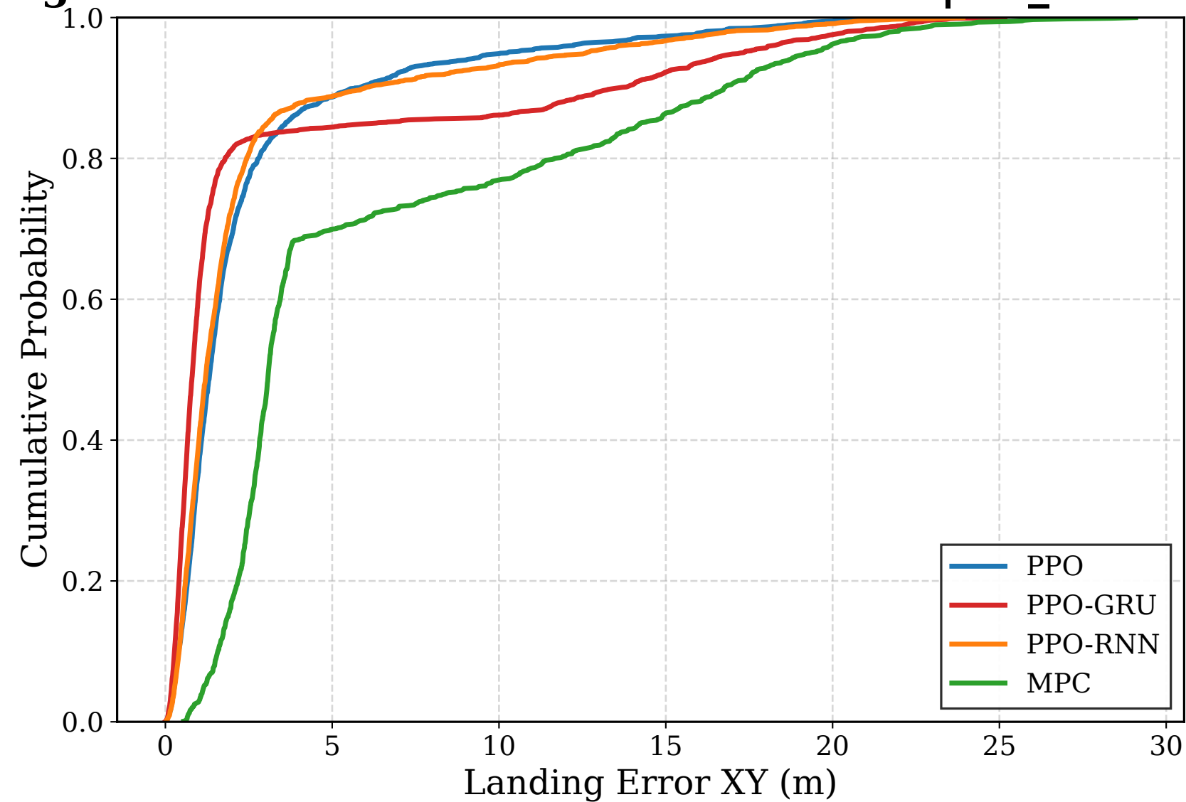
Experiment 2: Fixed Height + Fixed Wind + Obstacle Ablation | no_obstacle | Landing Precision CDF
