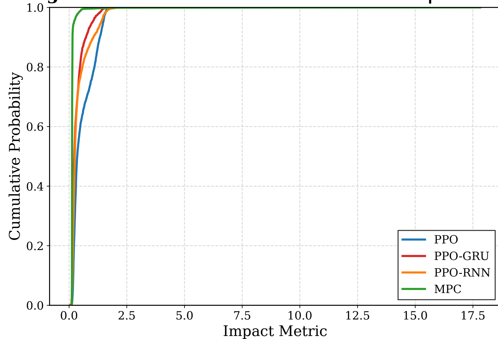
Experiment 2: Fixed Height + Fixed Wind + Obstacle Ablation | random_obstacle | Impact CDF
