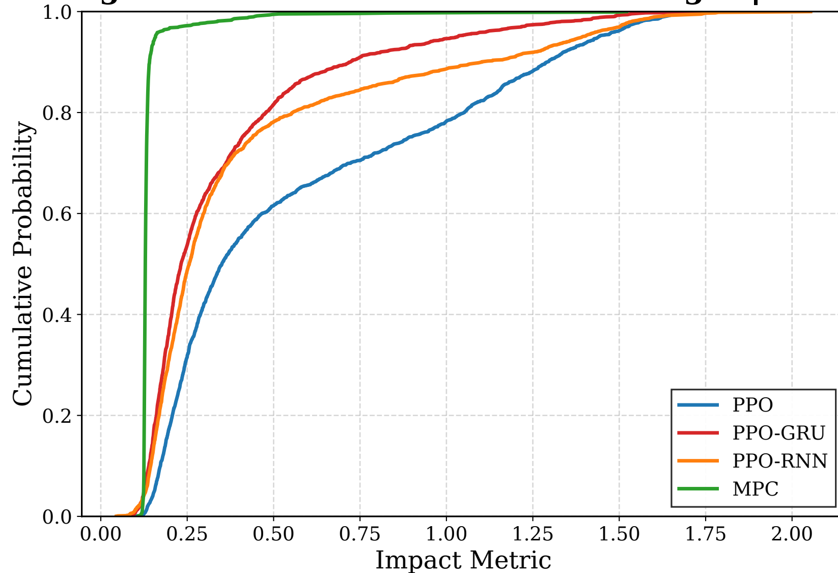
Experiment 4: Fixed Height + Obstacle + Multi Wind Strength | medium_wind | Impact CDF
