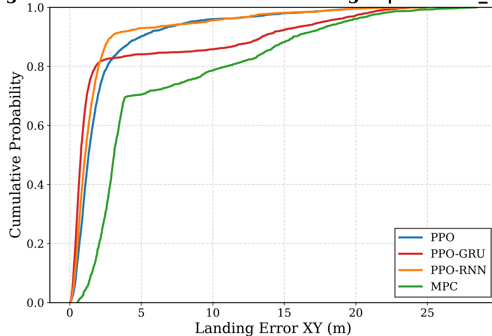
Experiment 4: Fixed Height + Obstacle + Multi Wind Strength | medium_wind | Landing Precision CDF
