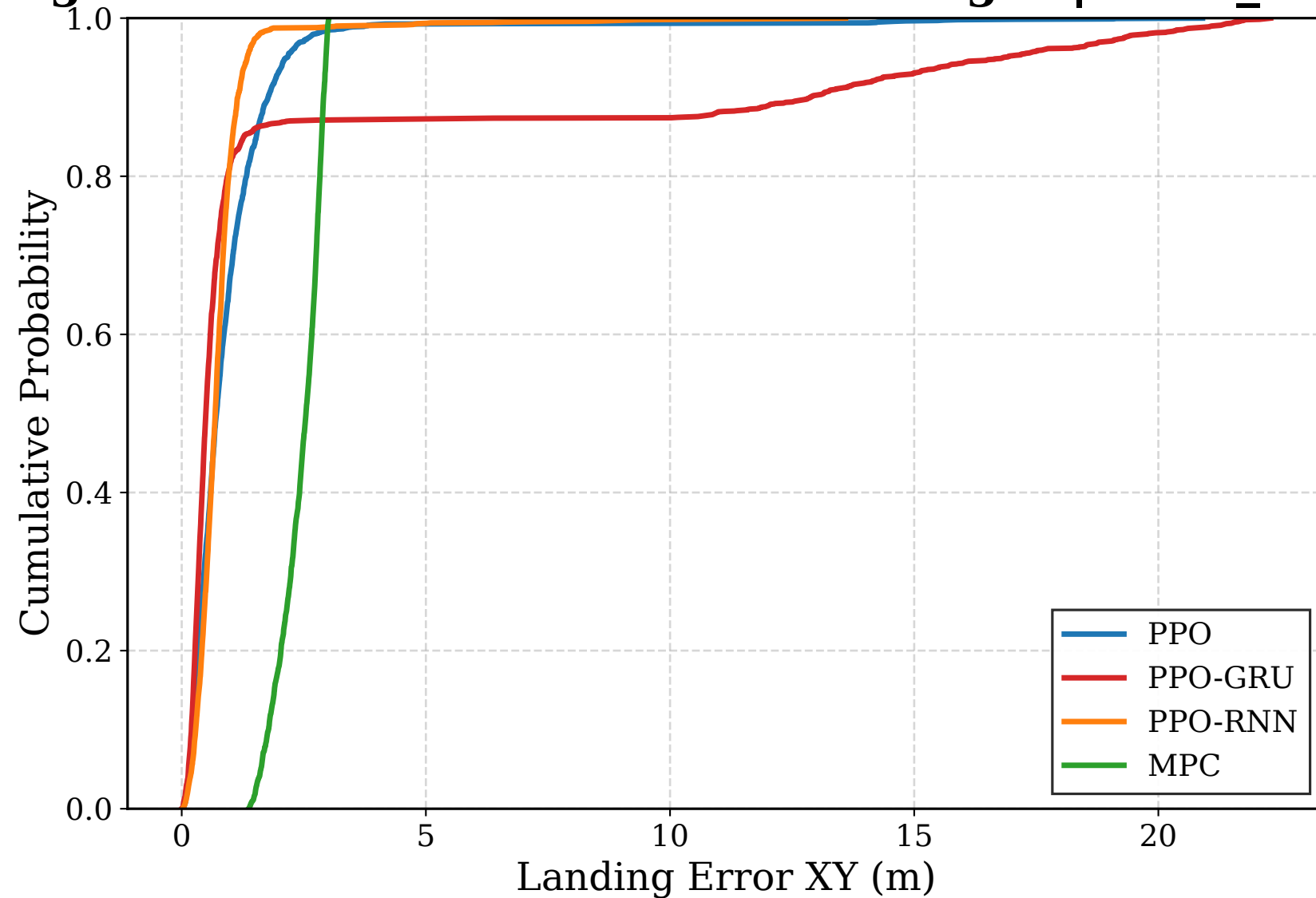
Experiment 4: Fixed Height + Obstacle + Multi Wind Strength | weak_wind | Landing Precision CDF
