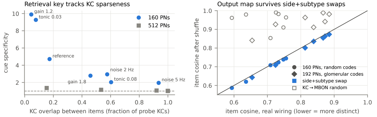
Fig. 8. Sensitivity to gain, tonic drive and membrane noise. Left: cue specificity of the written item (median over six write pairs) against the KC overlap between items, for seven parameter settings; dashed: no specificity. Right: mean pairwise cosine of item outputs with the real wiring against the same after swapping KC output profiles within subtype and side (filled) or randomising KC→MBON wiring (open), for the seven settings and two input codes; points on the diagonal keep the output map.
