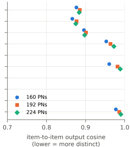
Bilateral glomerular symbol codes
