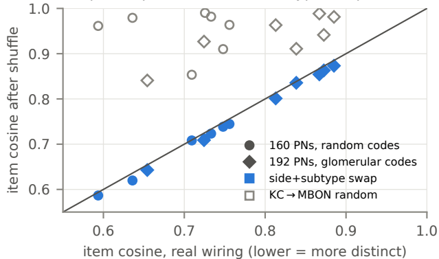
Output map survives side+subtype swaps
