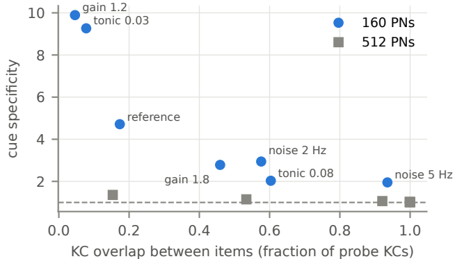
Retrieval key tracks KC sparseness
