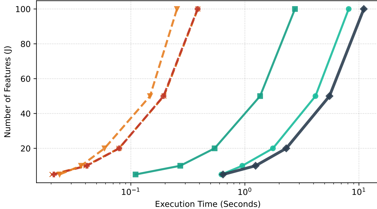
B. Scalability over Features (J)
