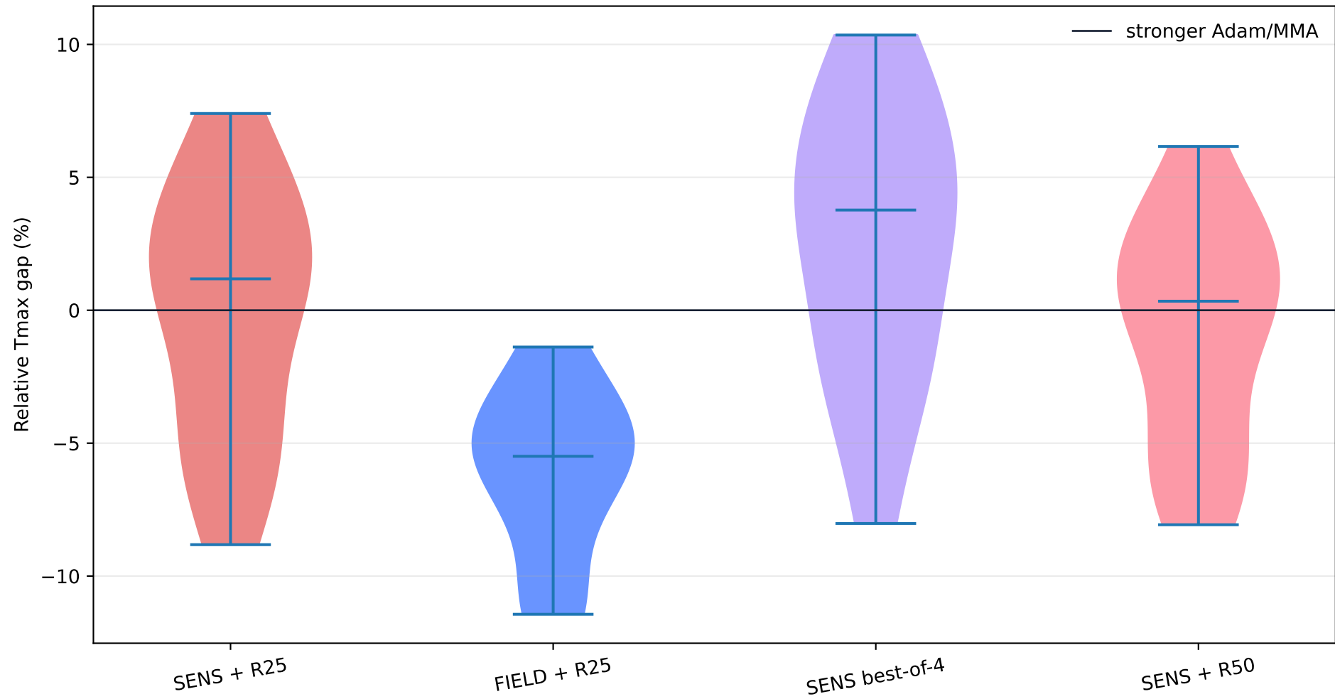
OOD quality distribution
