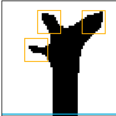
Head 0
