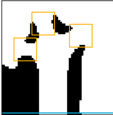
Head 1
