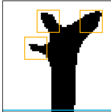
Head 2
