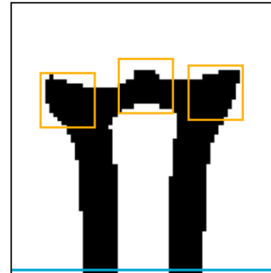
Head 3 (selected)
