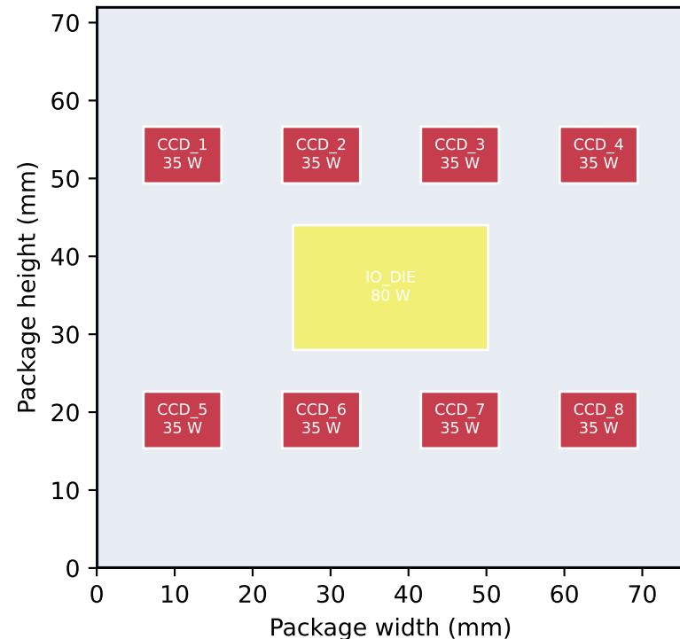
uniform_compute Total = 360 W
