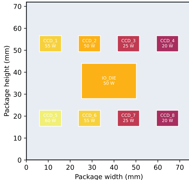
localized_compute Total = 360 W
