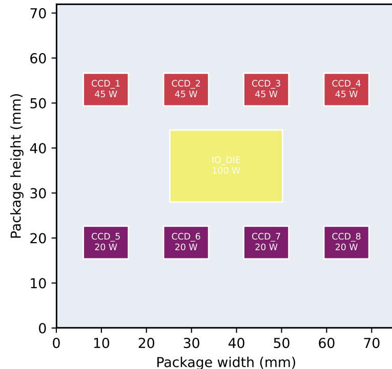
asymmetric_rows Total = 360 W
