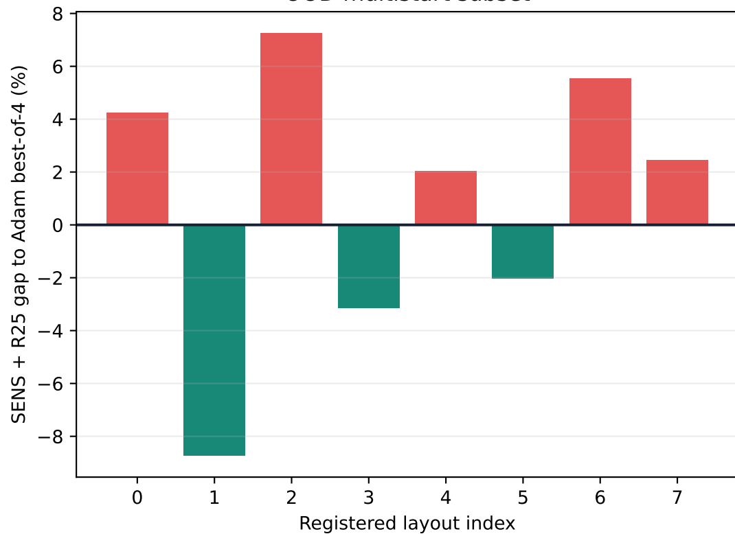
OOD multistart subset
