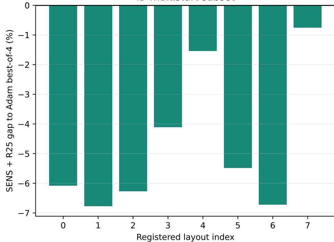
ID multistart subset
