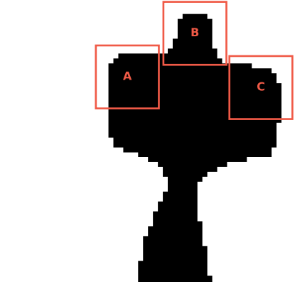
PHYSICS binary
