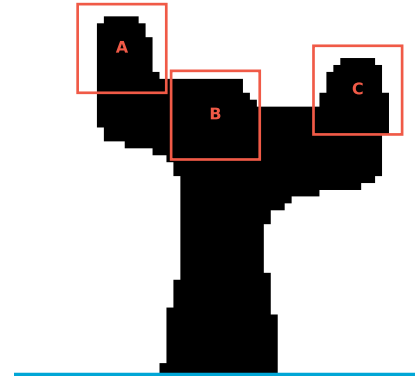
PHYSICS binary
