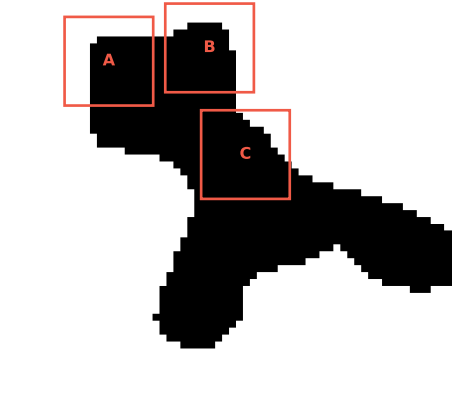
PHYSICS binary
