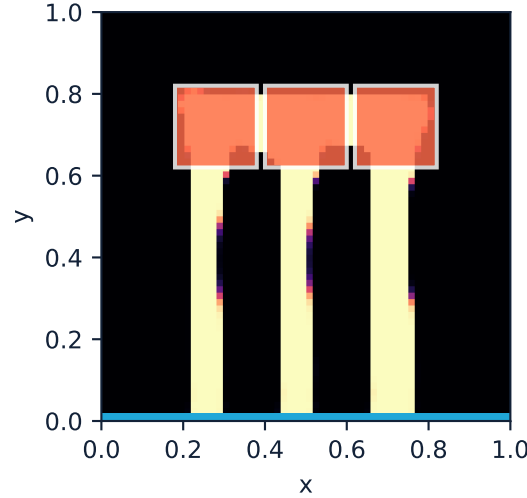
strict binary • Tmax=0.154835 effect PASS
