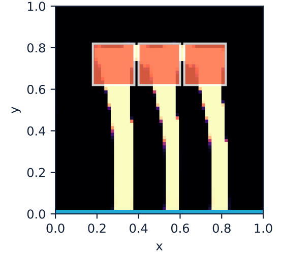
strict binary • Tmax=0.161150 effect PASS
