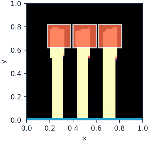
strict binary • Tmax=0.189398 catastrophic collapse
