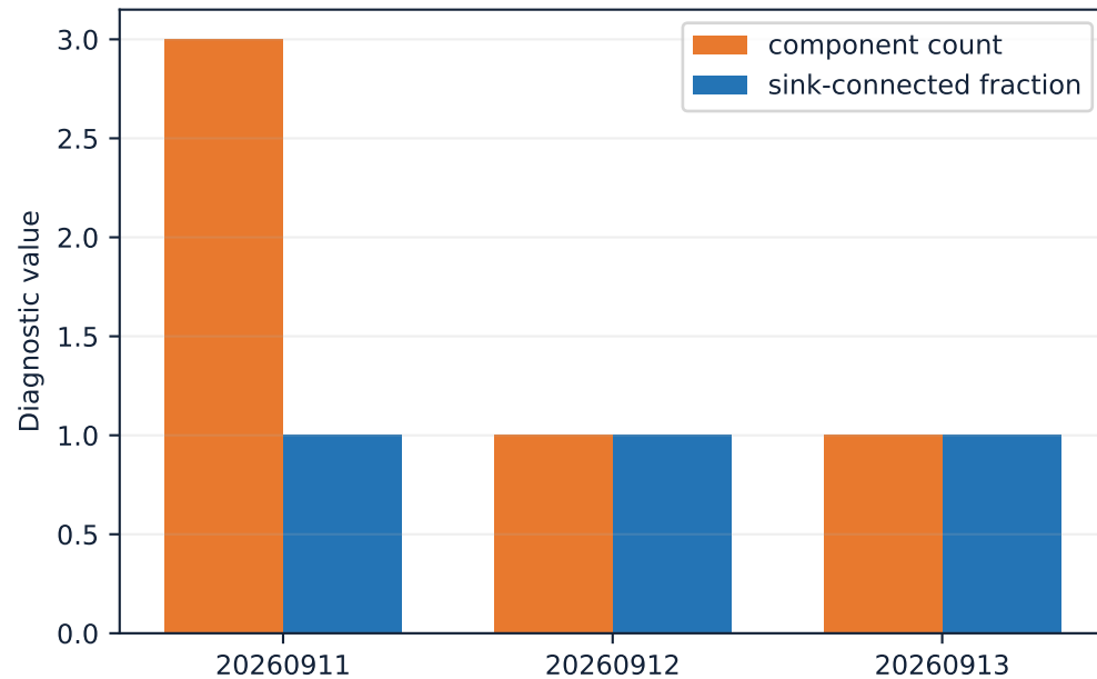
High-k connectivity
