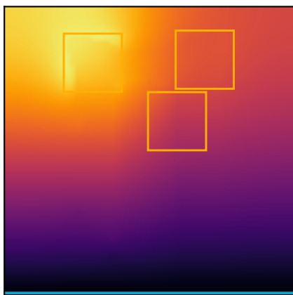
FIELD U-Net + R25 - scenario A Tmax=0.174510
