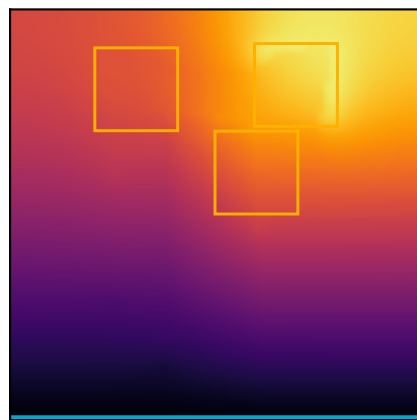
FIELD U-Net + R25 - scenario C Tmax=0.175706
