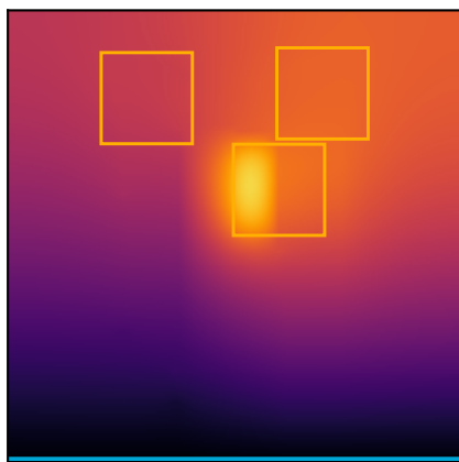
FIELD U-Net + R25 - scenario B Tmax=0.166554
