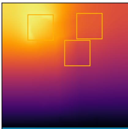
SENS U-Net + R25 - scenario A Tmax=0.176706
