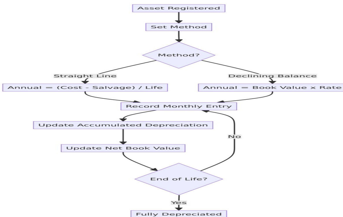
Figure 3: Complete Asset Lifecycle
