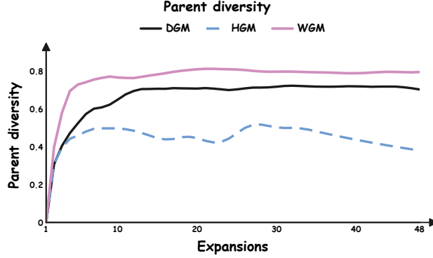
Figure 3: Lineage parent diversity during self-improvement. Parent diversity D(T) computed with the lineage indicator. The curves use the same search histories as Figure 1(b).
