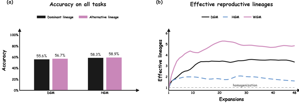
Figure 1: Reproductive-lineage diversity during self-improvement. (a) Accuracy of the best agent in the dominant lineage and in the alternative lineages. The alternative lineages contain agents that exceed the best agent of the dominant lineage. (b) Effective number of reproductive lineages L(T) (Eq. 3), computed from the parent-selection histories of the experiments with lineages. L(T) = 1 means that all parent selections come from a single lineage. DGM and HGM concentrate reproduction on a few lineages, whereas WGM keeps reproduction spread across more lineages. (See experimental setup in Appendix D.3).
