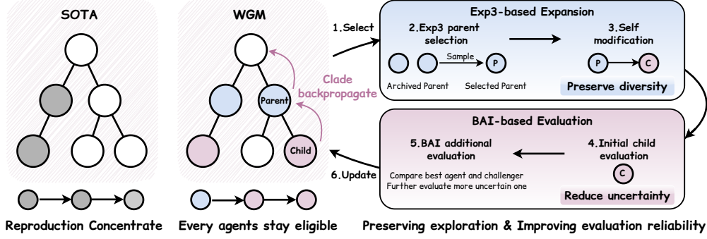
Figure 2: Overview of WGM. EXP3 selects parents using weights adjusted by clade statistics, while a uniform exploration floor keeps every archived agent eligible. BAI allocates additional evaluations across the archive and selects the final agent. Initial evaluations of new children update their parents’ EXP3 weights, and both initial and additional evaluations update clade statistics for subsequent parent selection.
