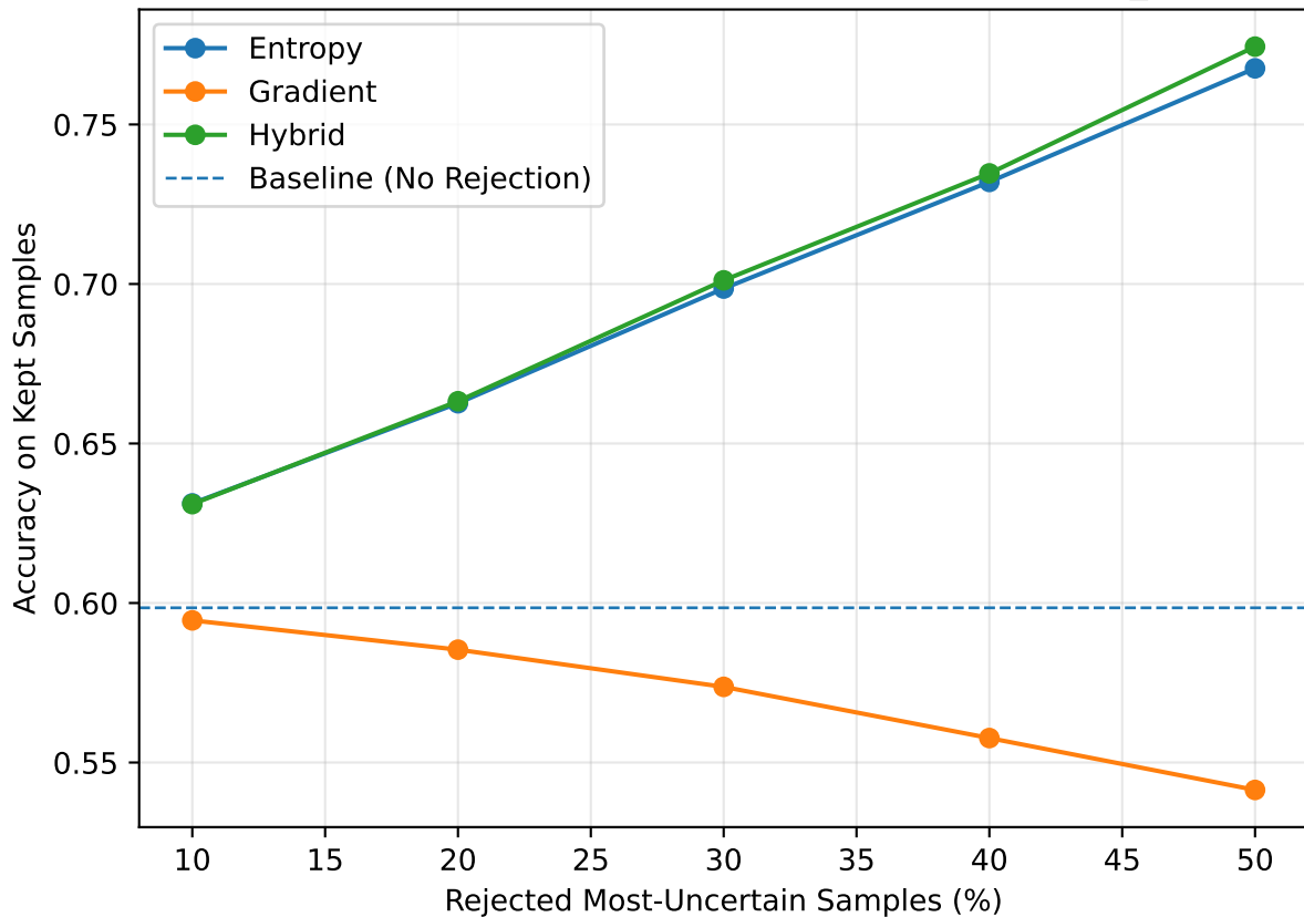
Accuracy vs Rejection — cifar10 / efficientnetv2_s
