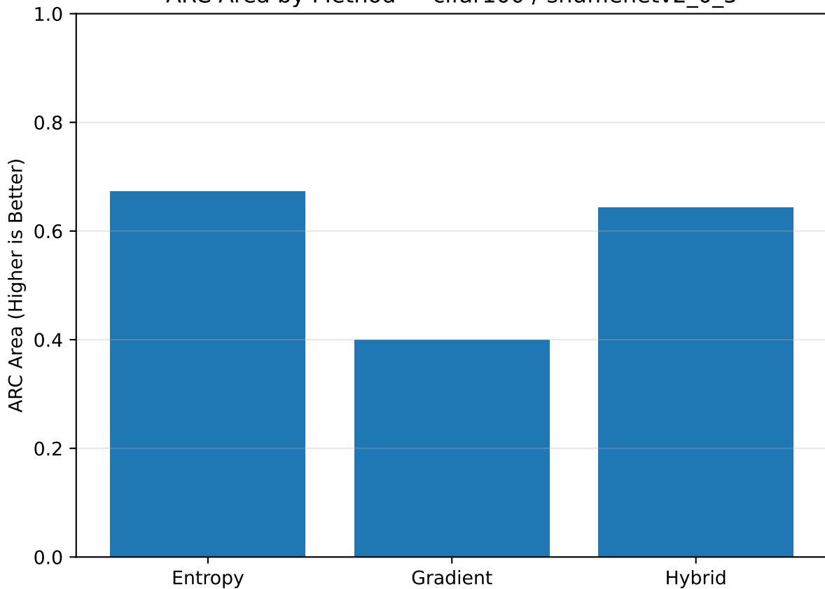
ARC Area by Method — cifar100 / shufflenetv2_0_5
