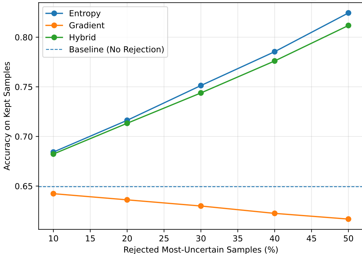
Accuracy vs Rejection — tissuemnist / mobilenetv3_small
