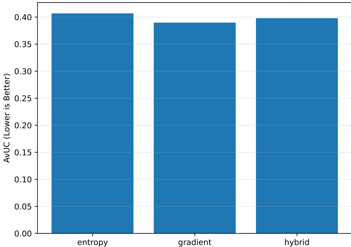
AvUC by Method — cifar10-c / shufflenetv2_0_5
