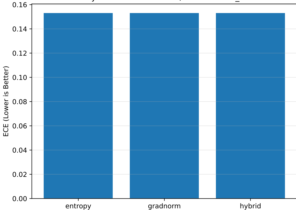
ECE by Method — cifar10-c / mobilenetv3_small
