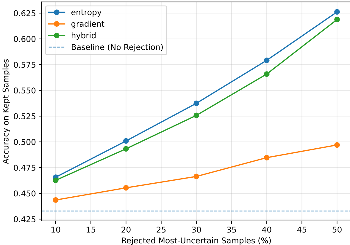
Accuracy vs Rejection — cifar100 / shufflenetv2_0_5
