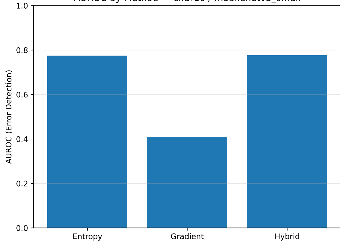
AUROC by Method — cifar10 / mobilenetv3_small
