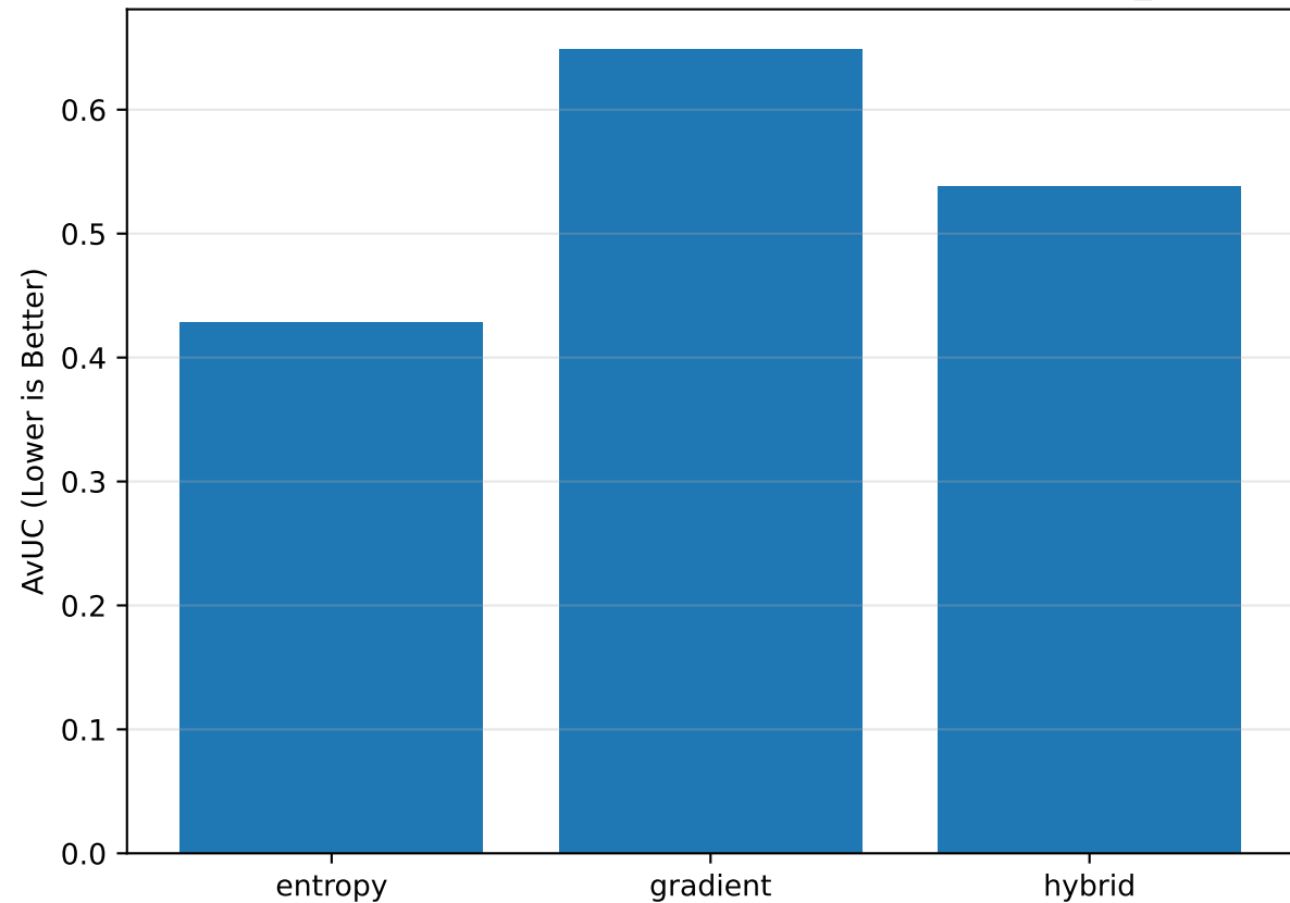
AvUC by Method — tinyimagenet-c / efficientnetv2_s
