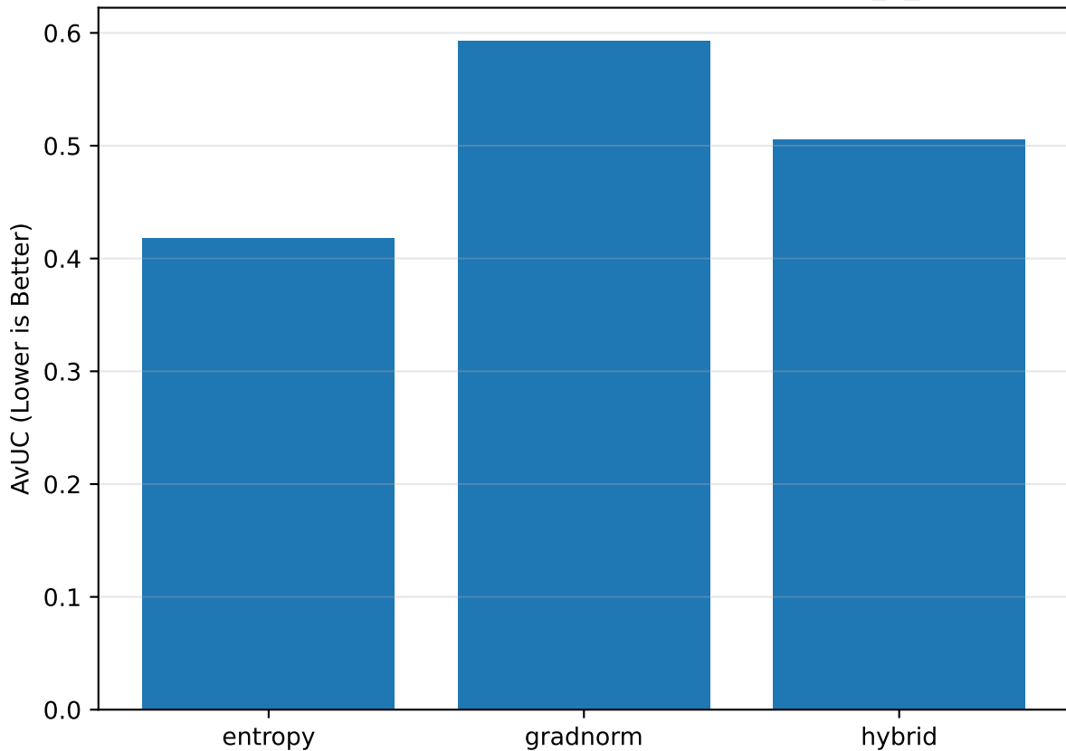
AvUC by Method — cifar100-c / shufflenetv2_0_5
