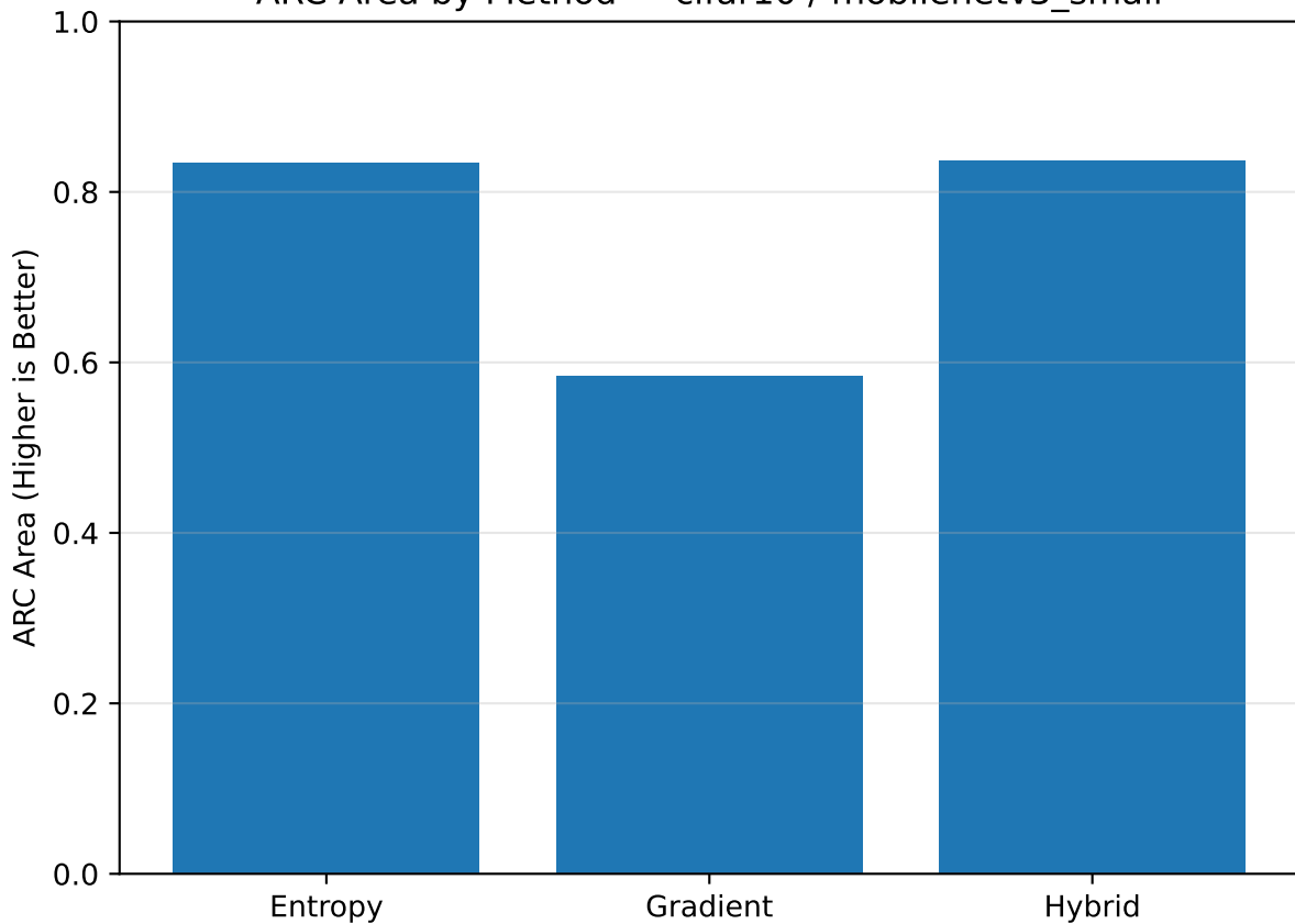
ARC Area by Method — cifar10 / mobilenetv3_small
