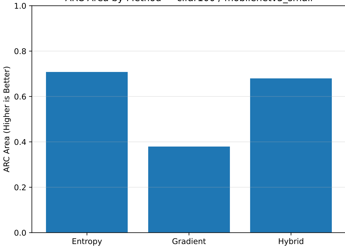
ARC Area by Method — cifar100 / mobilenetv3_small
