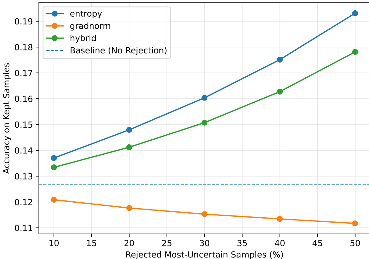
Accuracy vs Rejection — tinyimagenet-c / mobilenetv3_small
