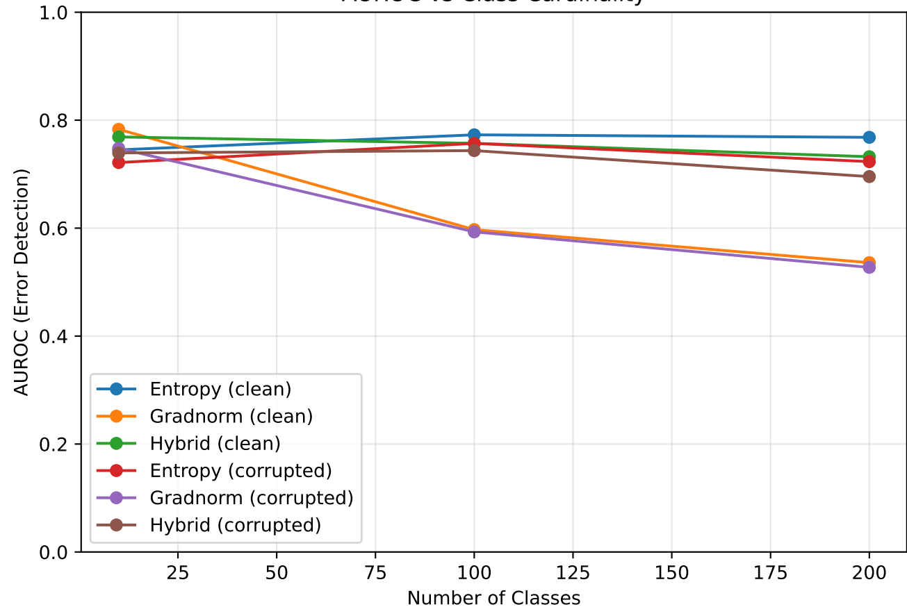
AUROC vs Class Cardinality
