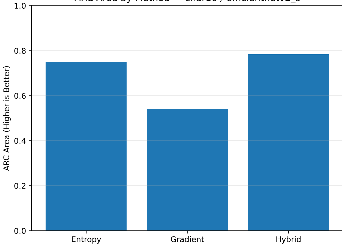
ARC Area by Method — cifar10 / efficientnetv2_s
