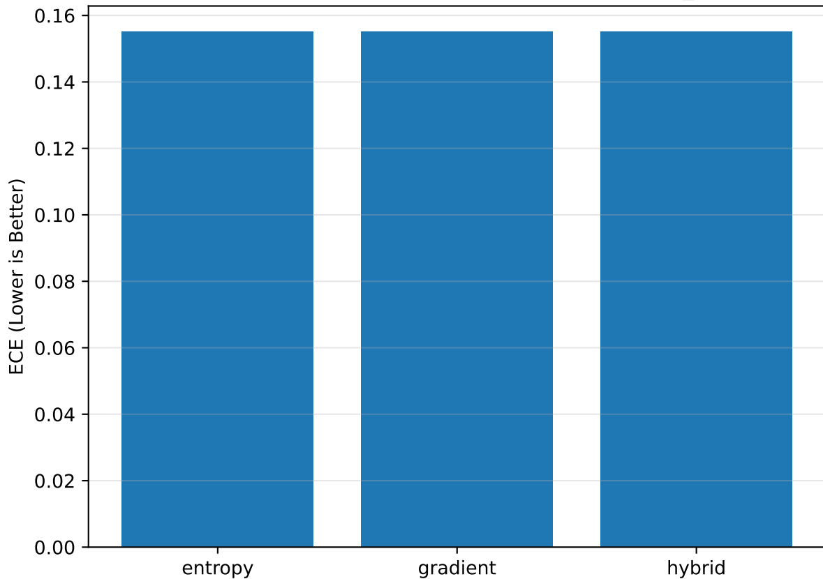
ECE by Method — cifar100 / efficientnetv2_s
