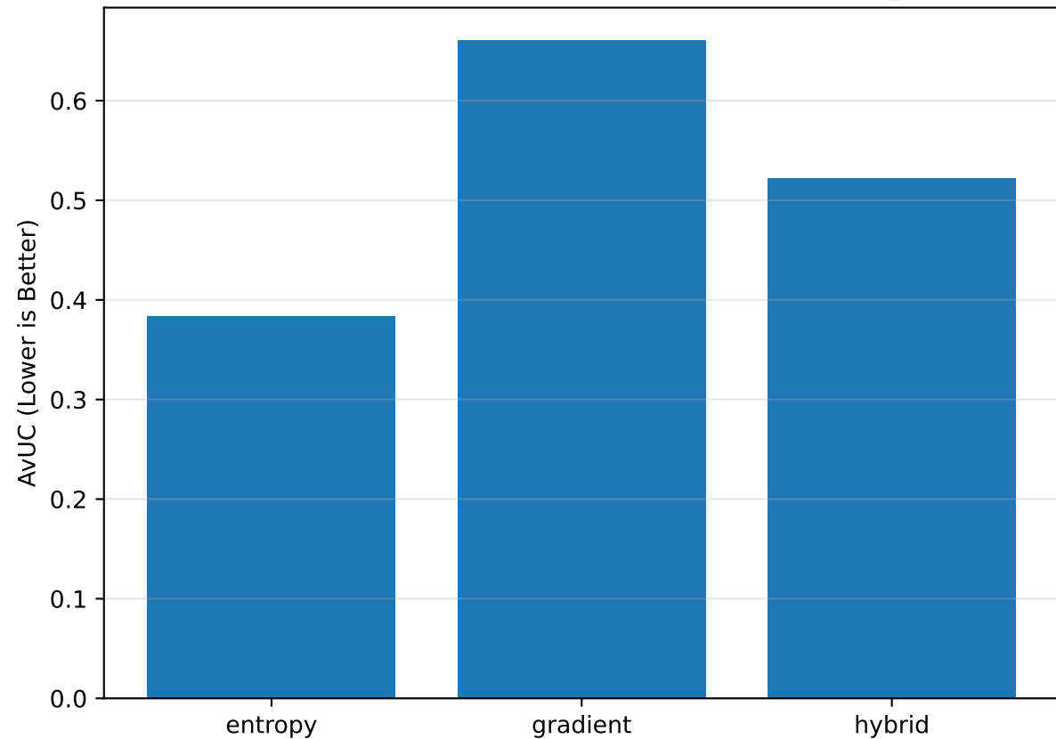
AvUC by Method — tinyimagenet-c / mobilenetv3_small
