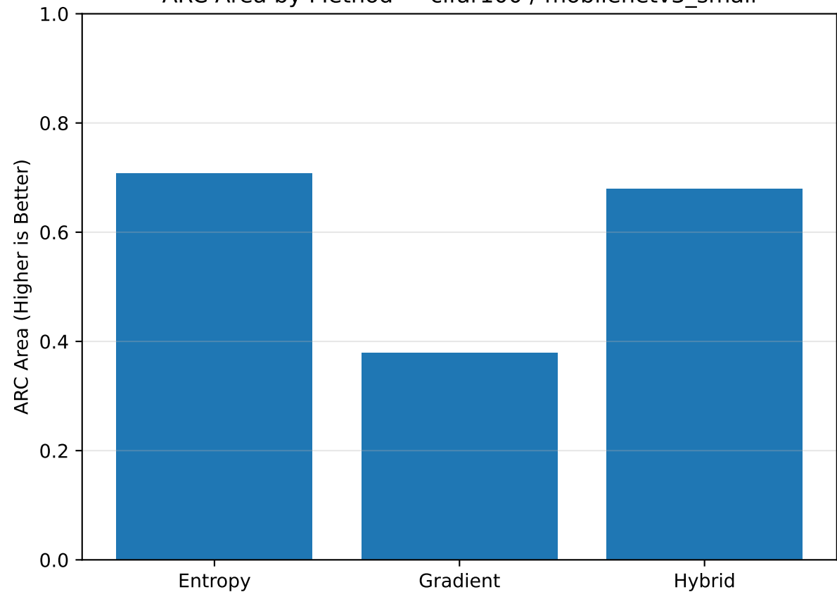
ARC Area by Method — cifar100 / mobilenetv3_small
