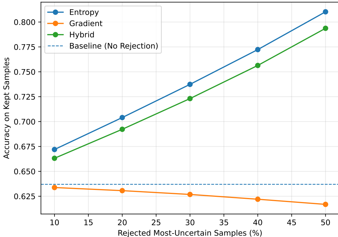
Accuracy vs Rejection — tissuemnist / shufflenetv2_0_5
