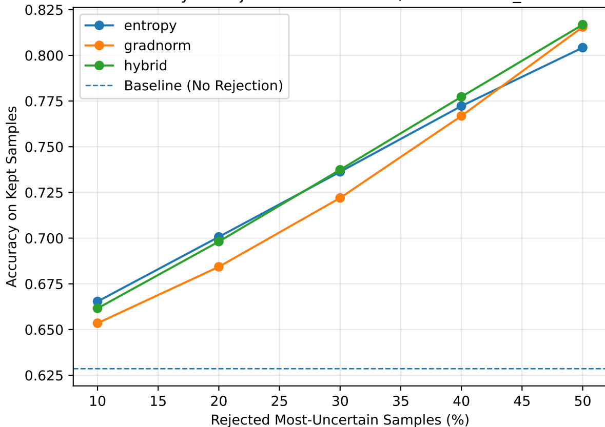
Accuracy vs Rejection — cifar10-c / mobilenetv3_small
