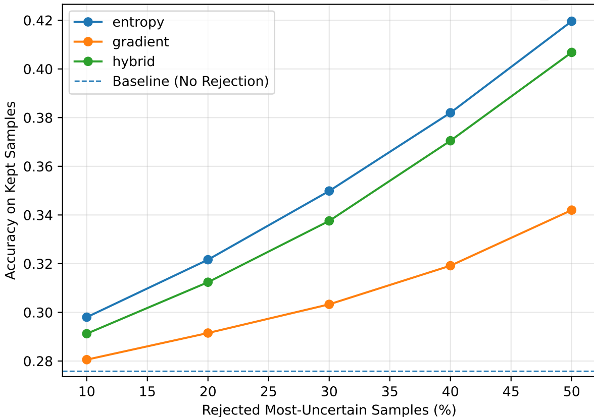
Accuracy vs Rejection — tinyimagenet / efficientnetv2_s
