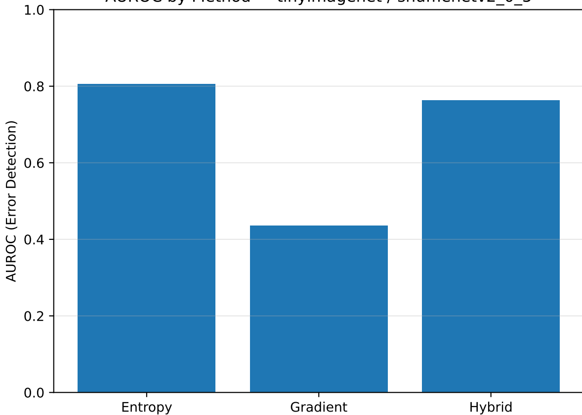
AUROC by Method — tinyimagenet / shufflenetv2_0_5
