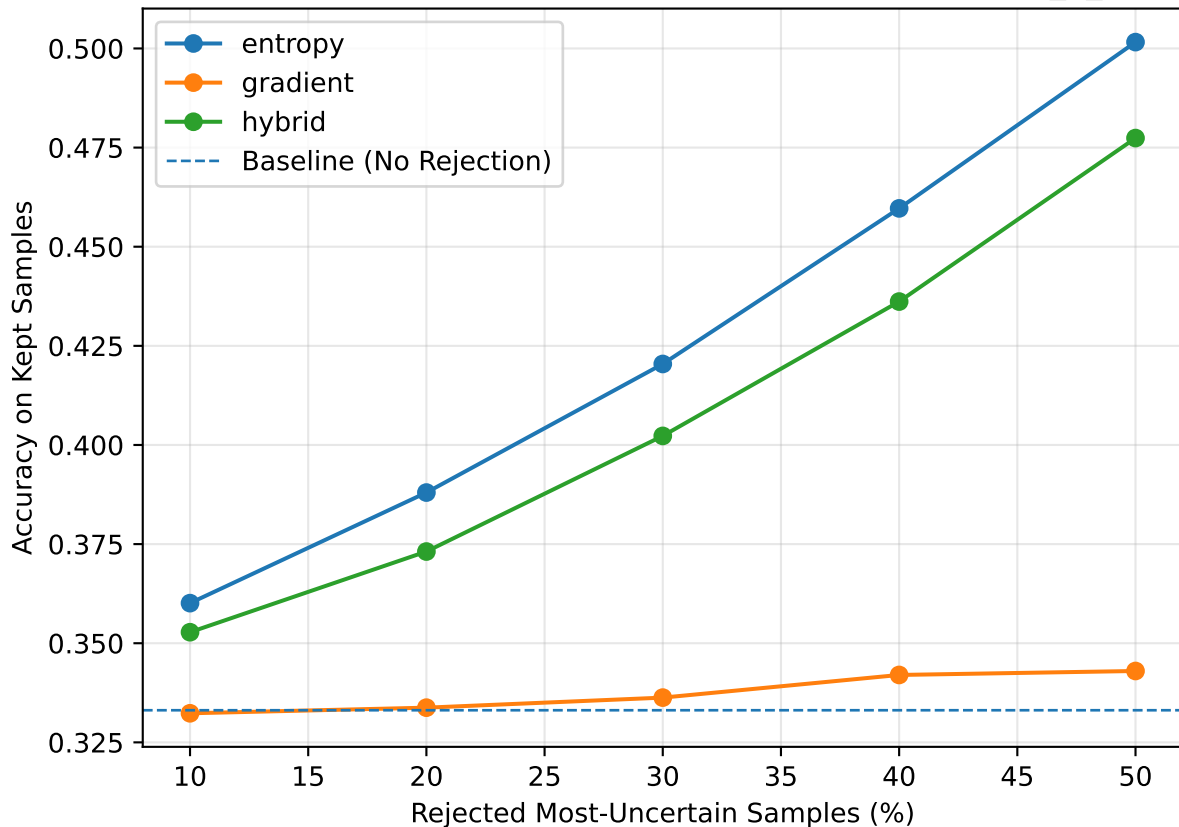
Accuracy vs Rejection — tinyimagenet / shufflenetv2_0_5
