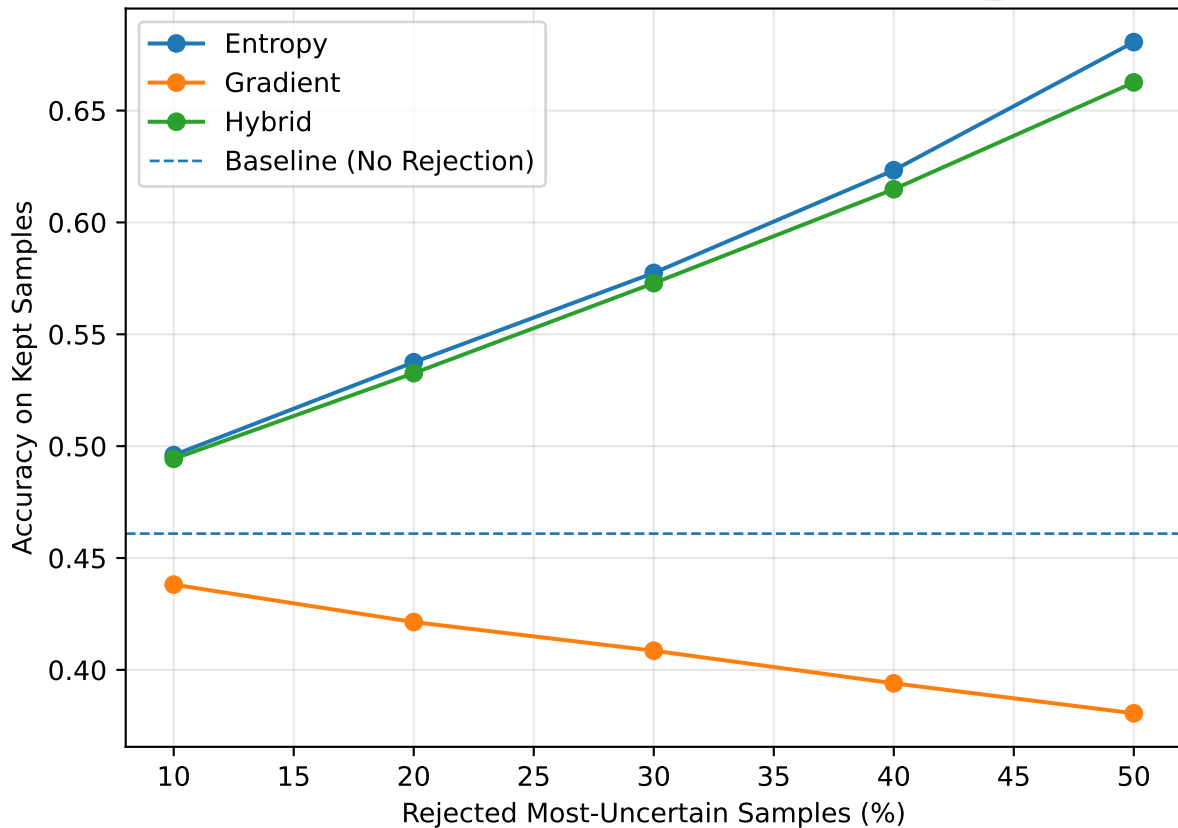
Accuracy vs Rejection — cifar100 / mobilenetv3_small
