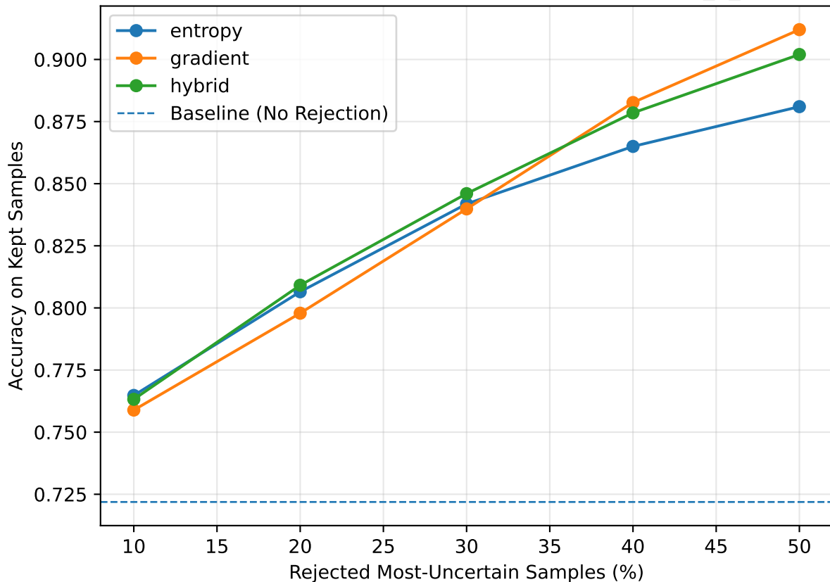
Accuracy vs Rejection — cifar10 / shufflenetv2_0_5
