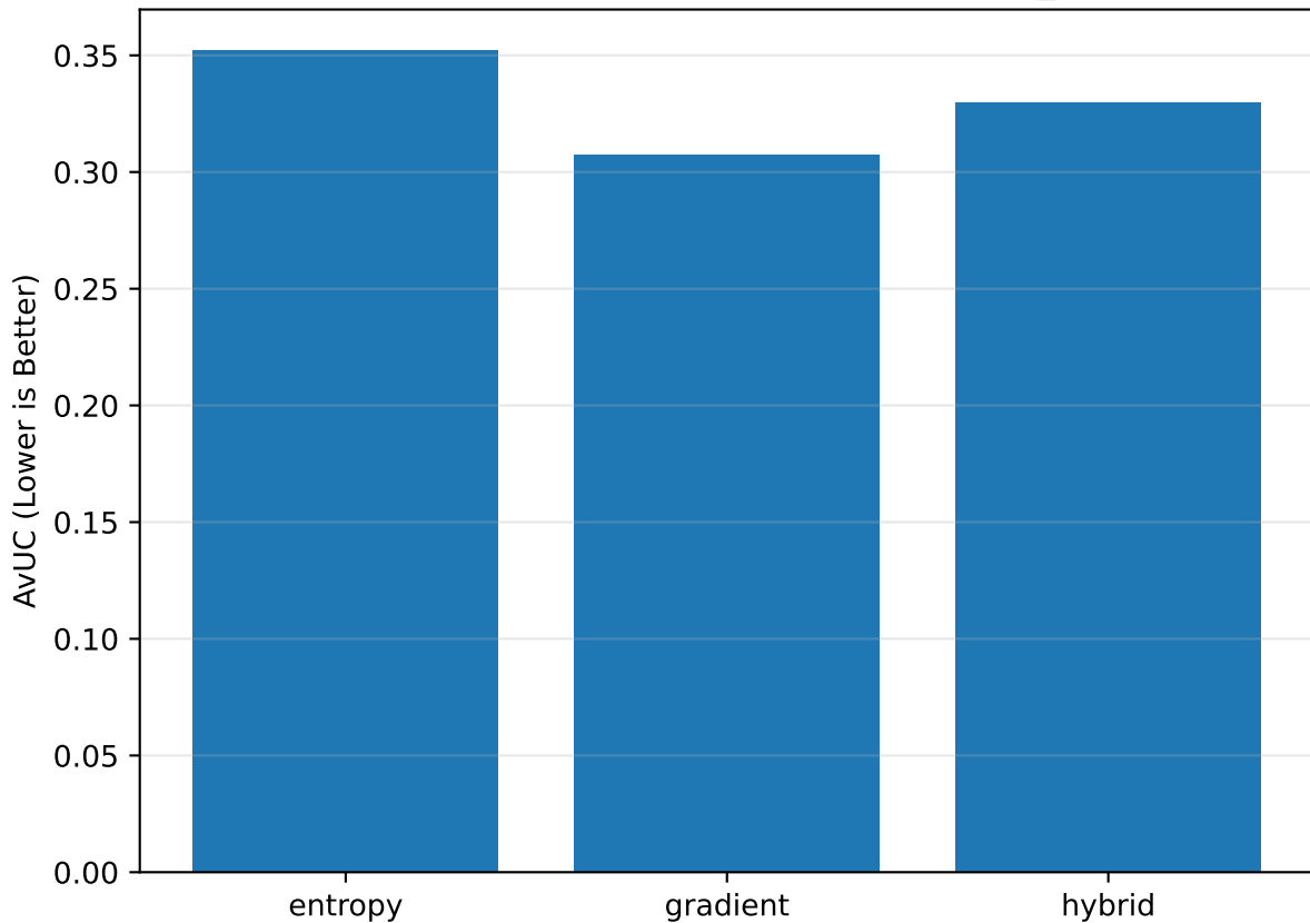
AvUC by Method — cifar10 / mobilenetv3_small
