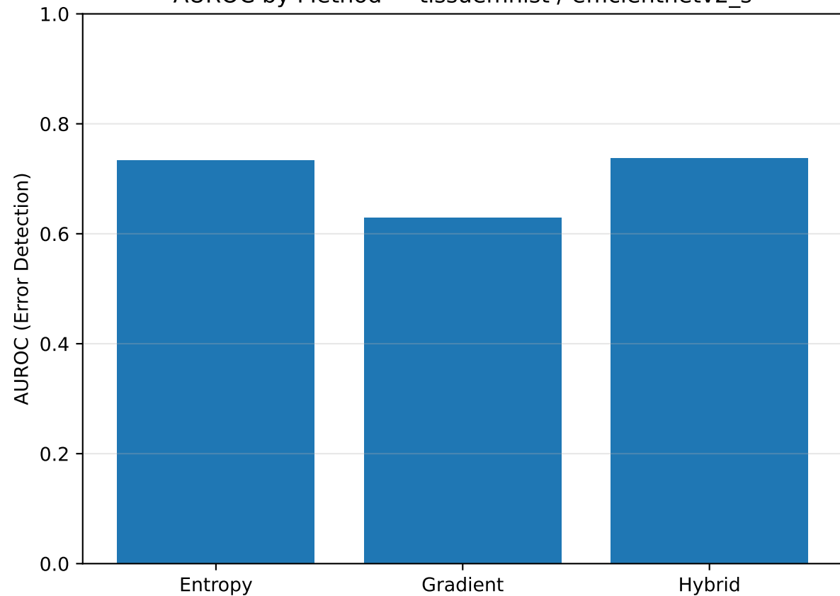
AUROC by Method — tissuemnist / efficientnetv2_s
