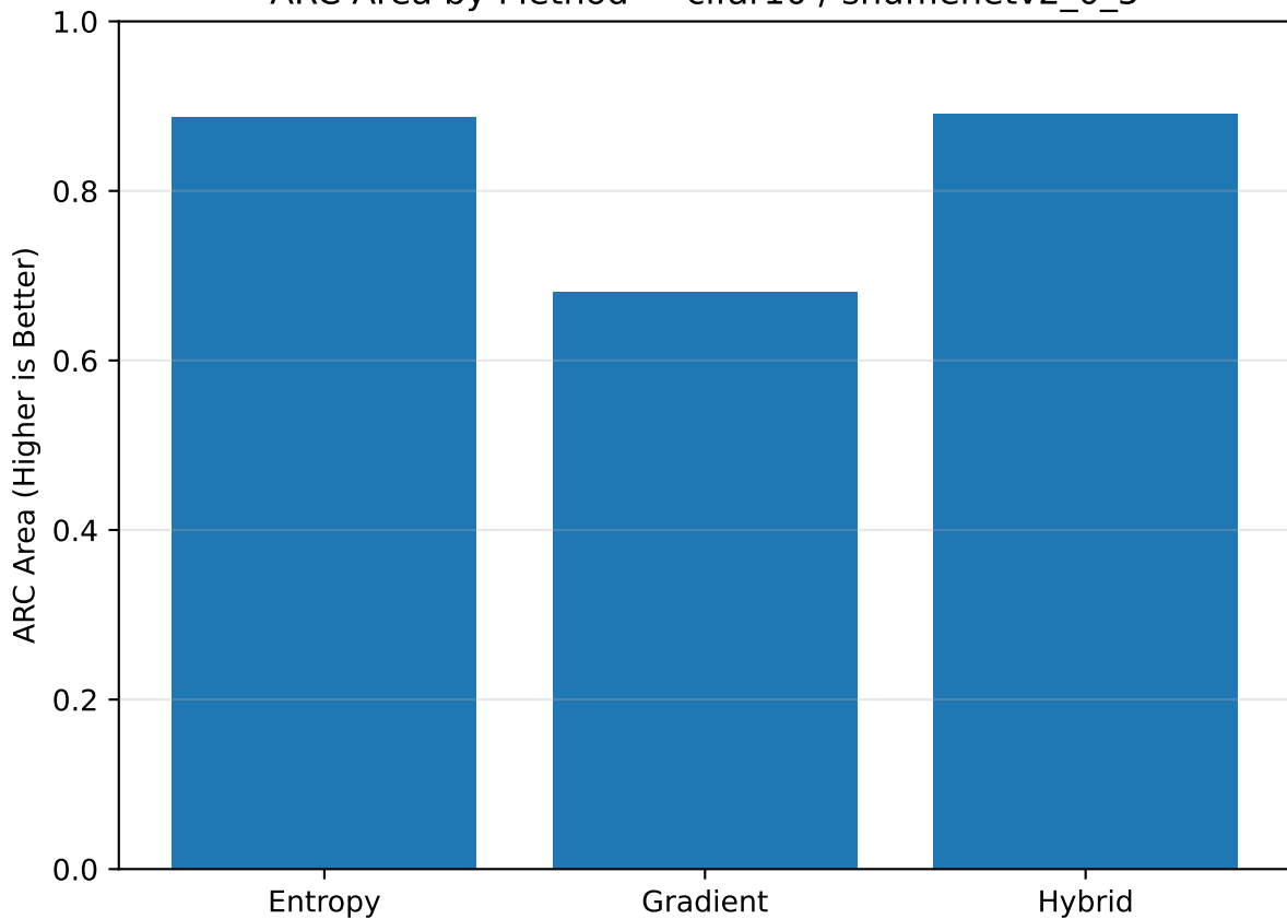
ARC Area by Method — cifar10 / shufflenetv2_0_5
