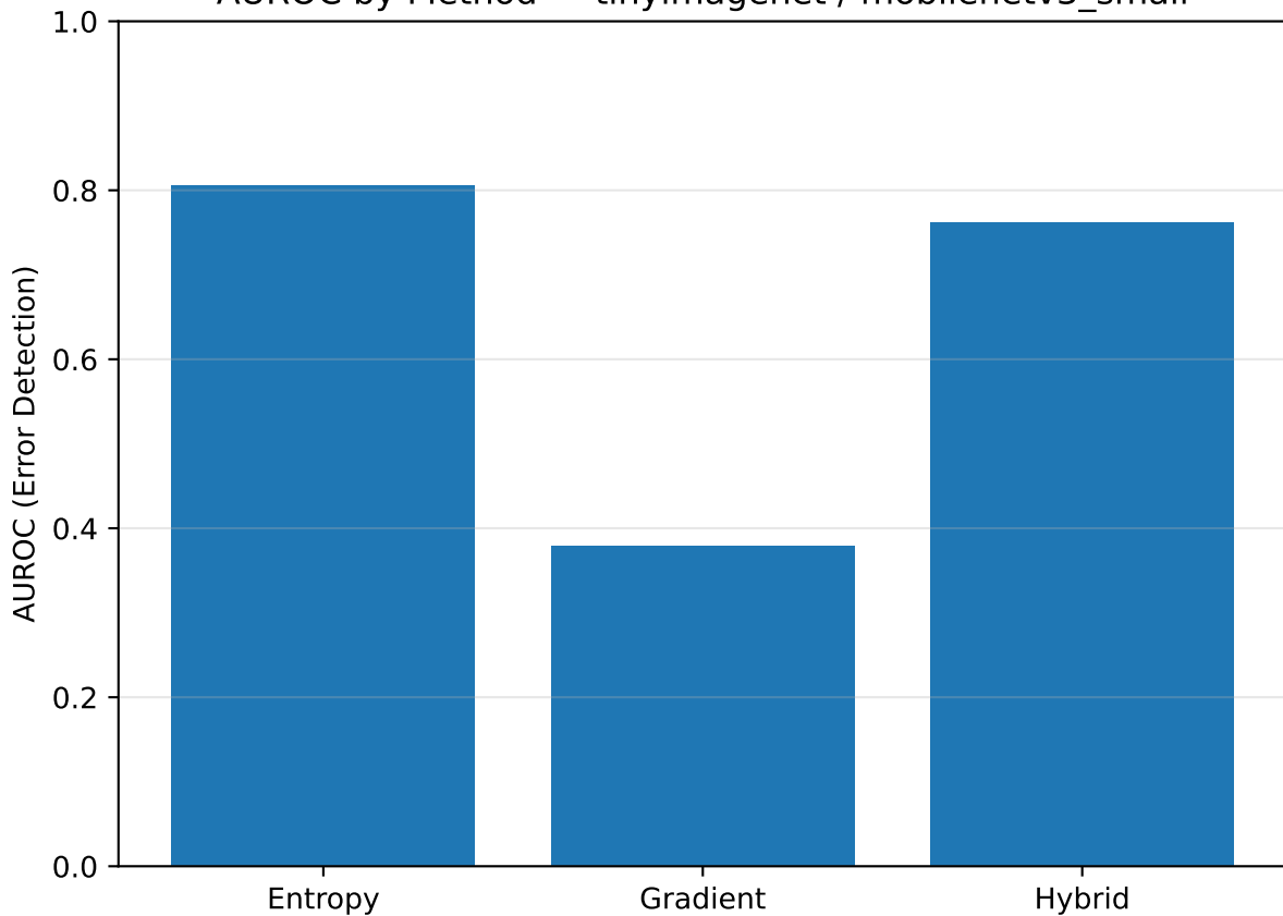
AUROC by Method — tinyimagenet / mobilenetv3_small
