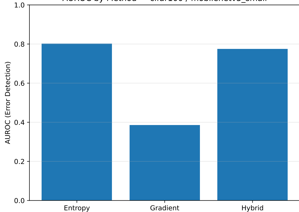
AUROC by Method — cifar100 / mobilenetv3_small
