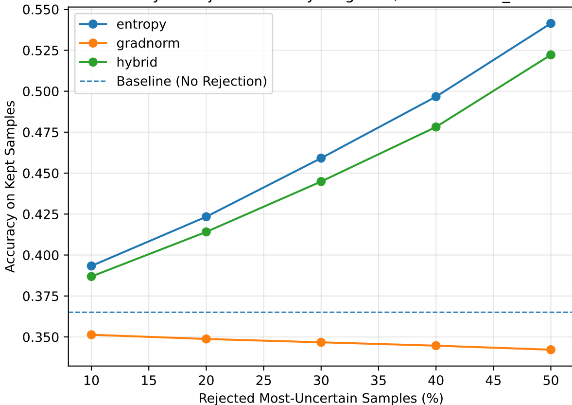
Accuracy vs Rejection — tinyimagenet / mobilenetv3_small
