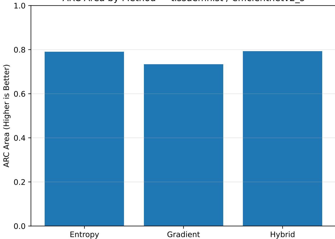
ARC Area by Method — tissuemnist / efficientnetv2_s
