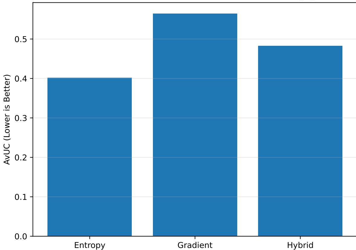
AvUC by Method — tinyimagenet / shufflenetv2_0_5
