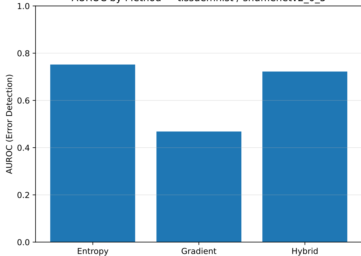
AUROC by Method — tissuemnist / shufflenetv2_0_5
