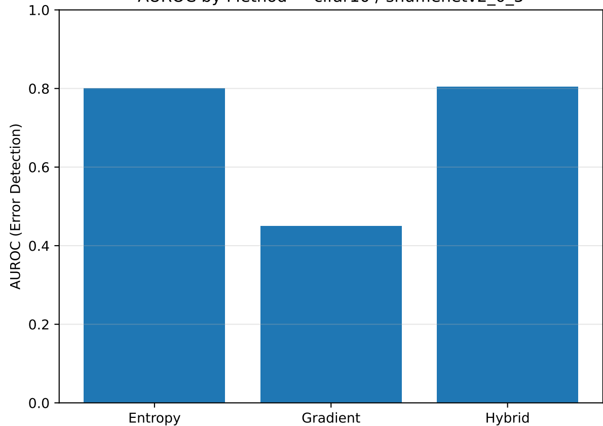
AUROC by Method — cifar10 / shufflenetv2_0_5
