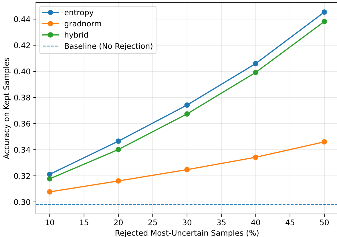
Accuracy vs Rejection — cifar100-c / shufflenetv2_0_5
