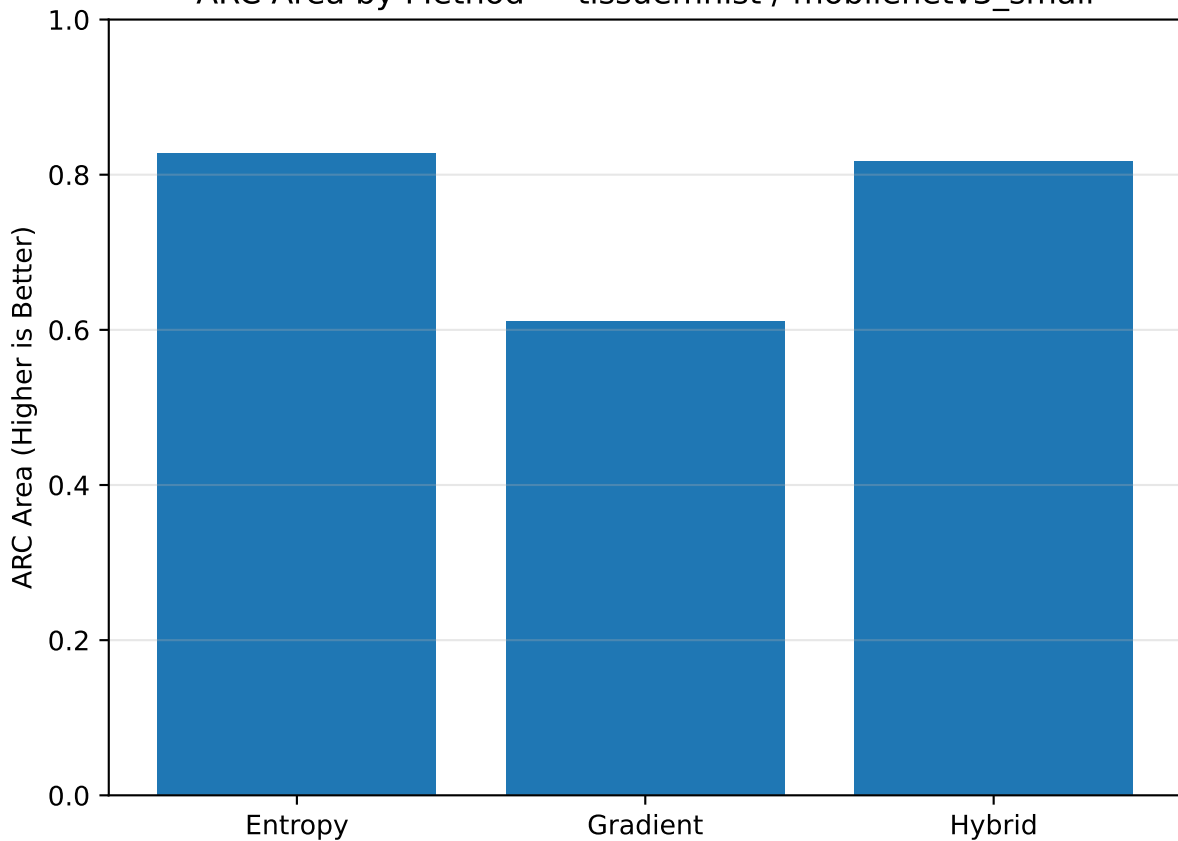
ARC Area by Method — tissuemnist / mobilenetv3_small
