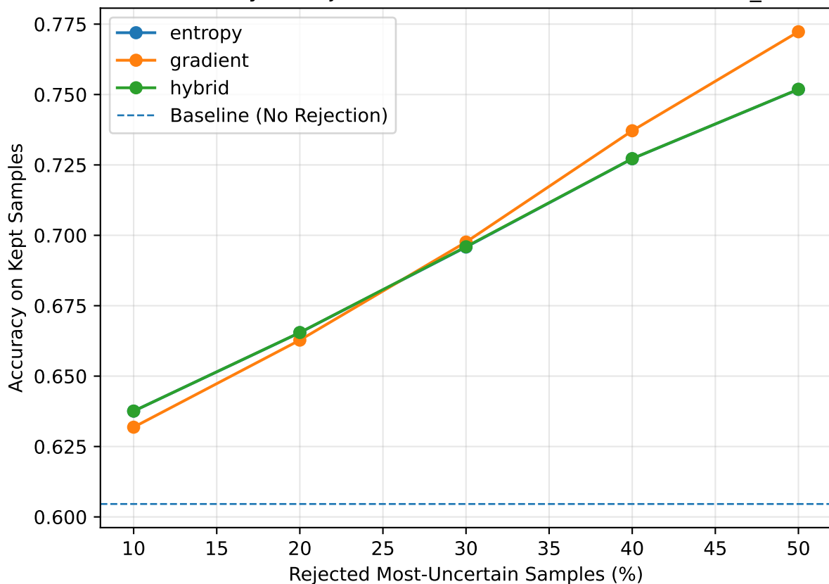
Accuracy vs Rejection — tissuemnist / efficientnetv2_s
