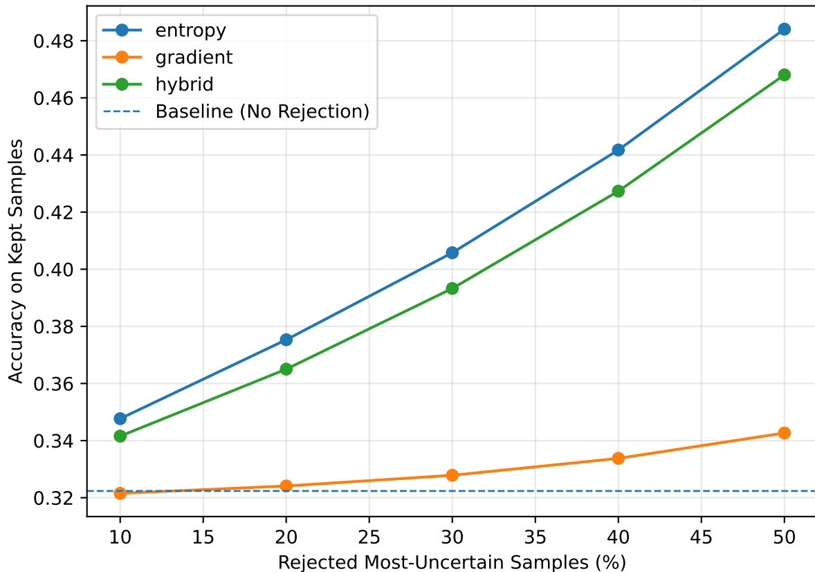
Accuracy vs Rejection — cifar100-c / mobilenetv3_small
