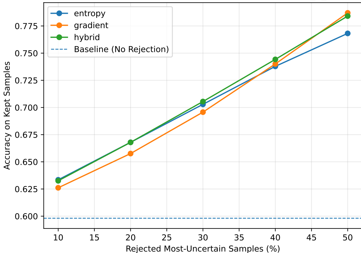
Accuracy vs Rejection — cifar10-c / shufflenetv2_0_5
