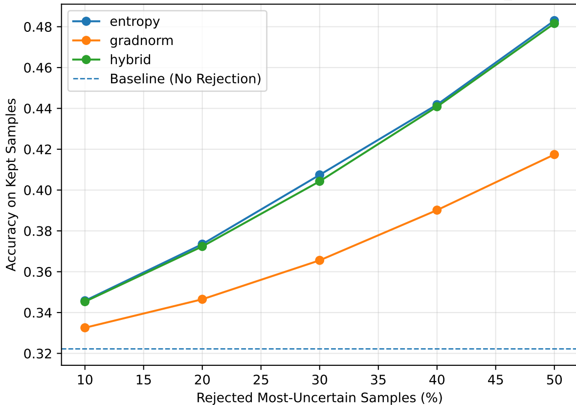
Accuracy vs Rejection — cifar100 / efficientnetv2_s
