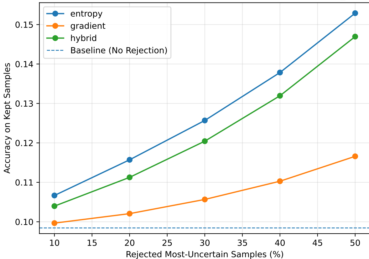
Accuracy vs Rejection — tinyimagenet-c / efficientnetv2_s
