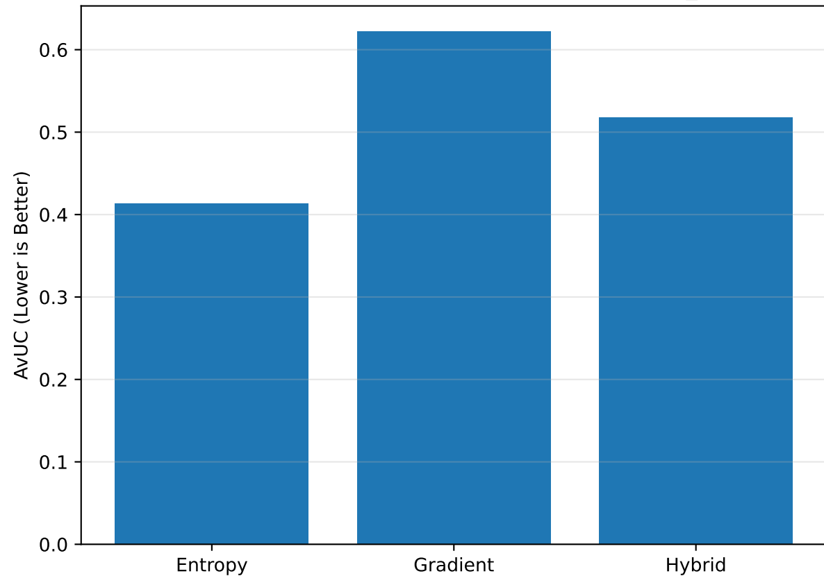
AvUC by Method — cifar100 / efficientnetv2_s
