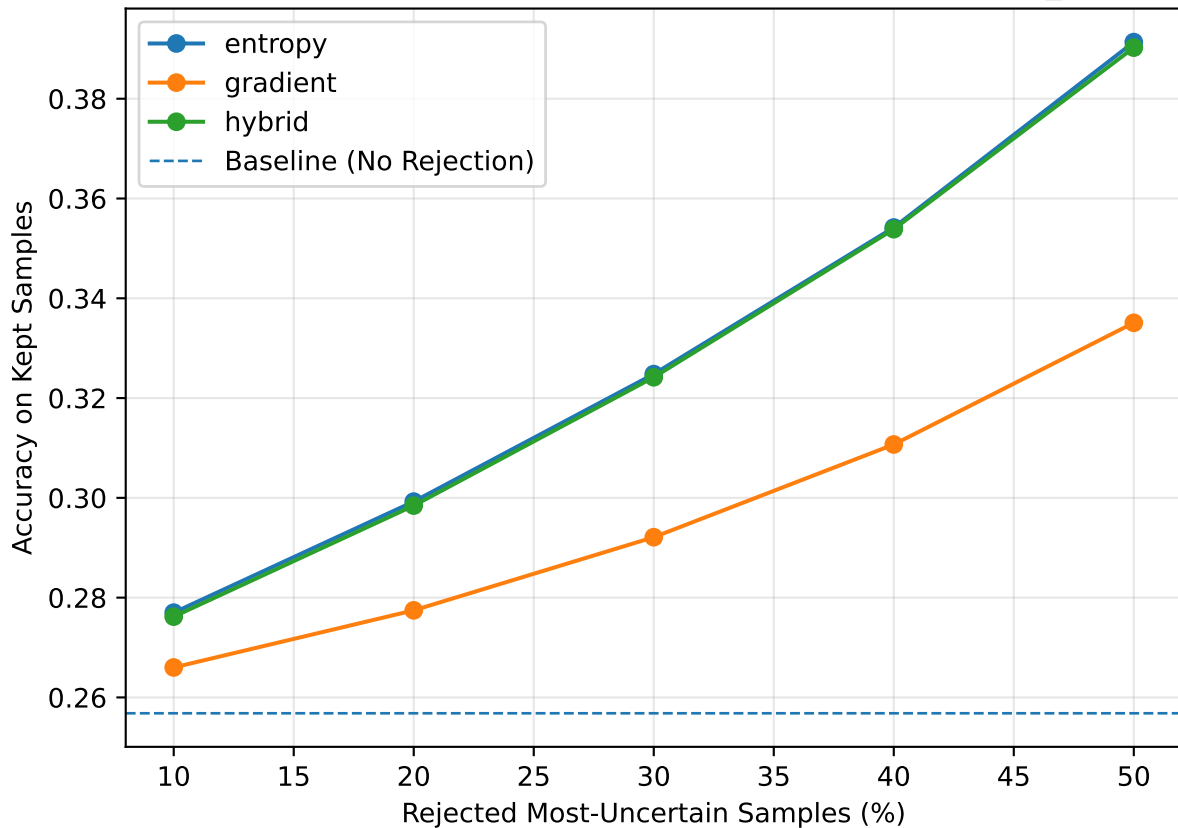
Accuracy vs Rejection — cifar100-c / efficientnetv2_s
