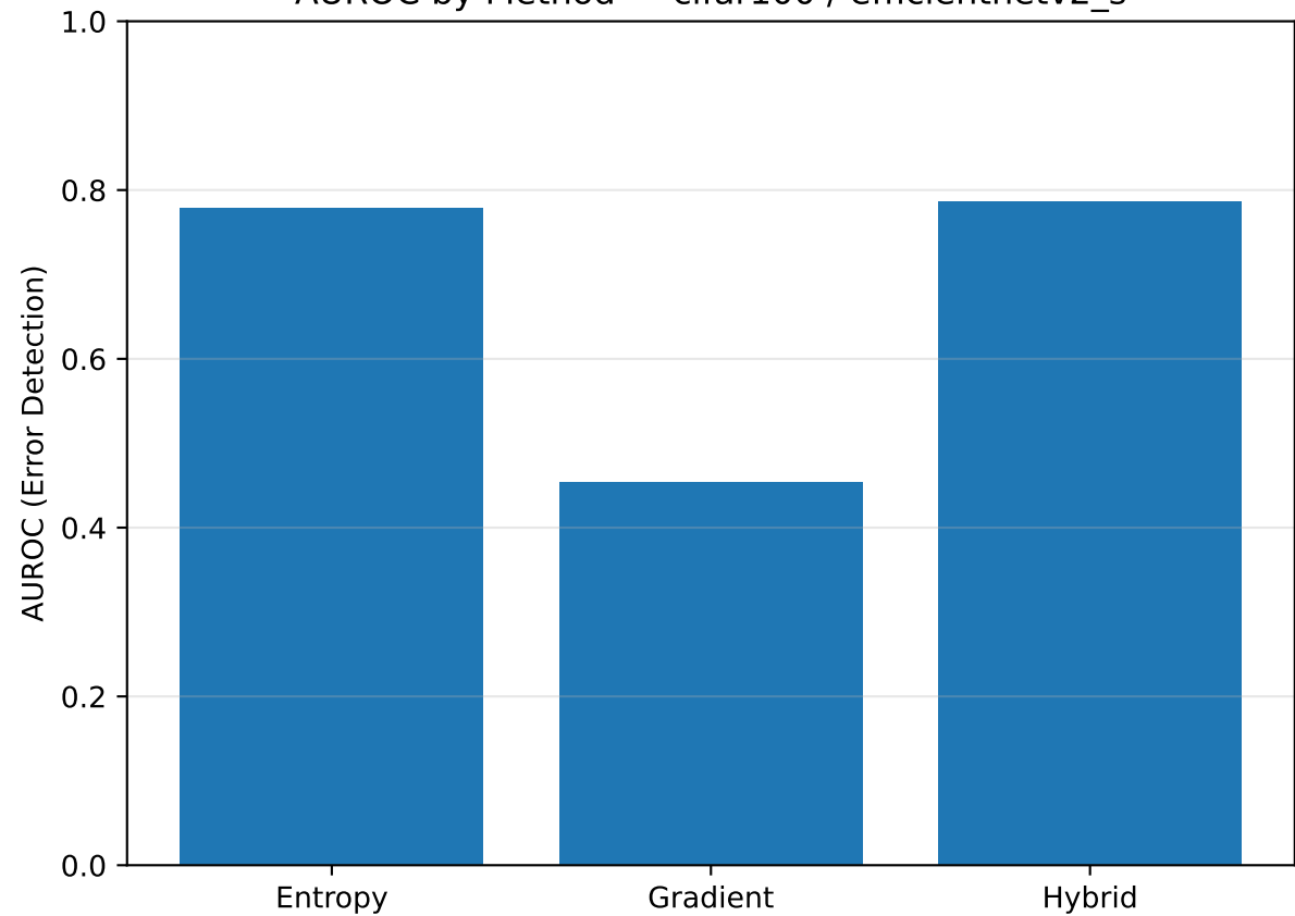
AUROC by Method — cifar100 / efficientnetv2_s
