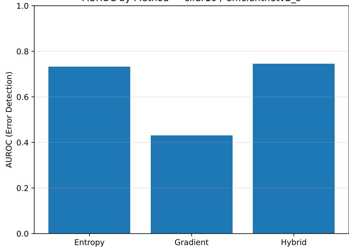
AUROC by Method — cifar10 / efficientnetv2_s
