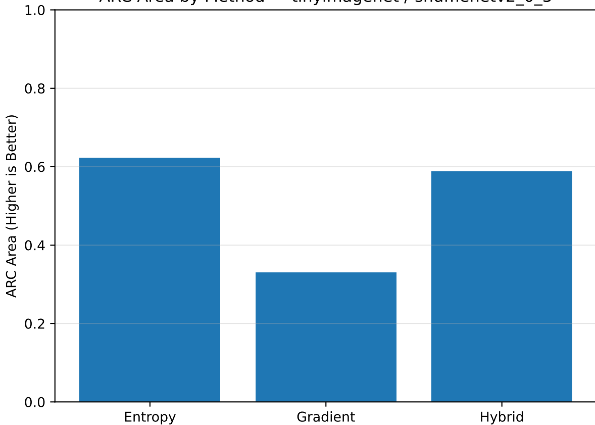
ARC Area by Method — tinyimagenet / shufflenetv2_0_5
