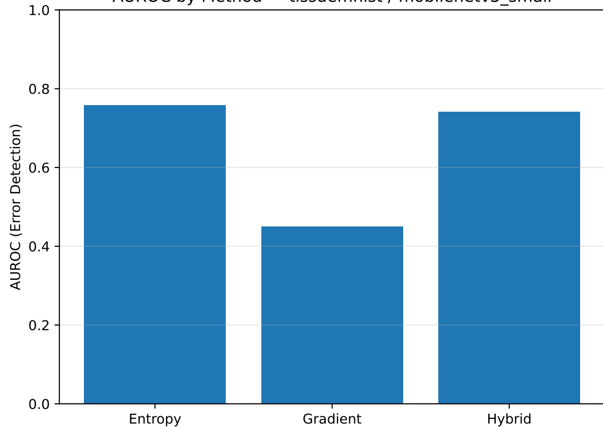
AUROC by Method — tissuemnist / mobilenetv3_small
