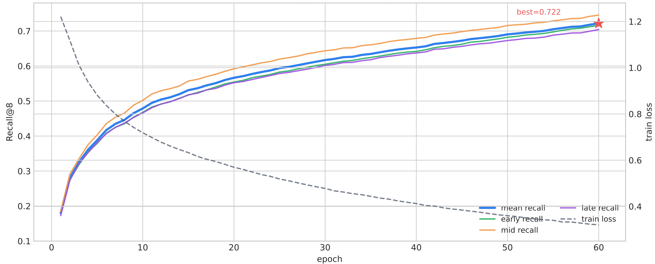
Global route predictor training curve
