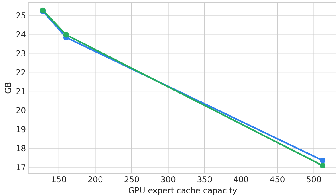
Transfer under lookahead=3
