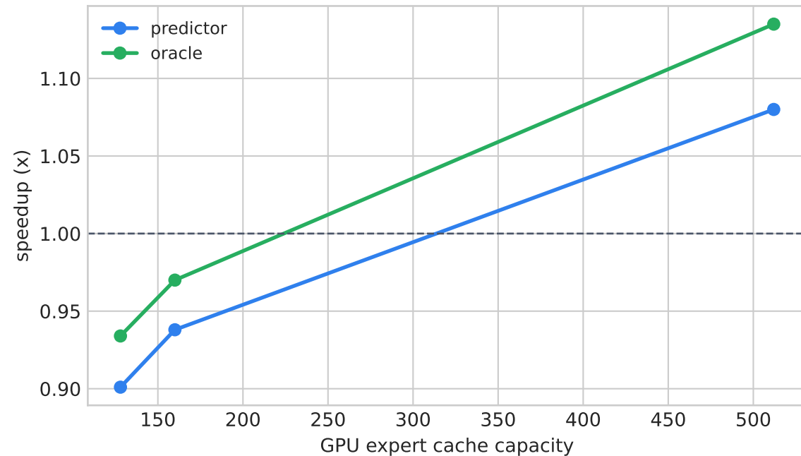
Speedup under lookahead=3
