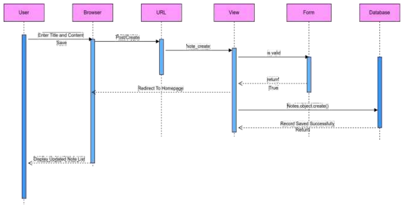
Fig 2. Sequence Diagram.
