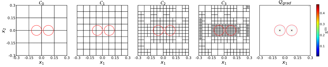
Figure 9: Example 4.4: Two circle sources: grid division diagram for IA-RFM with \delta = 10\% , M_0 = 2400 , Tanh, R_m = 5 . The last one shows the \mathcal{Q}_{\text{grad}} with t_{\text{grad}}=1/3 . The red dashed lines indicate the detected boundary, while the “x” symbols denote the detected center.
