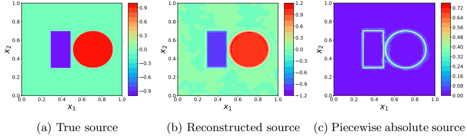
Figure 12: Example 4.5: One rectangle and one circle: Reconstruction with \delta = 5\% , M_0 = 1600 , M_1 = M_2 = 2400 , N_s = 10 and \lambda_{\text{reg}}^2 = 1 \times 10^{-3} yielding 15.28% E_{l^2}(S) using MA-RFM.
