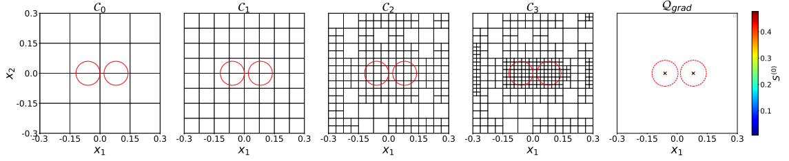
Figure 8: Example 4.4: Two circle sources: grid division diagram for IA-RFM with \delta = 10\% , M_0 = 2400 , Tanh, R_m = 5 . The last one shows the Q_{\text{grad}} with t_{\text{grad}}=1/3 . The red dashed lines indicate the detected boundary, while the “x” symbols denote the detected center.
