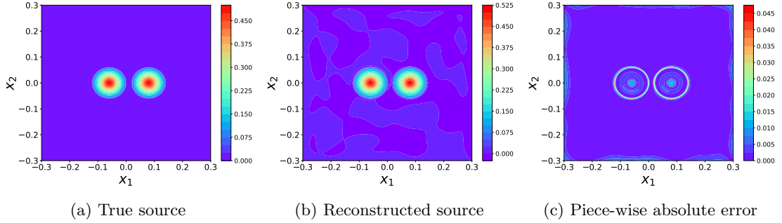
Figure 9: Example 4.4: Two circle sources: MA-RFM results with \delta = 10\% , M_{\text{total}} = 6400 , N_s = 20 and \lambda_{\text{reg}}^2 = 1 \times 10^{-4} yield an 4.64\% E_{l^2}(S) .
