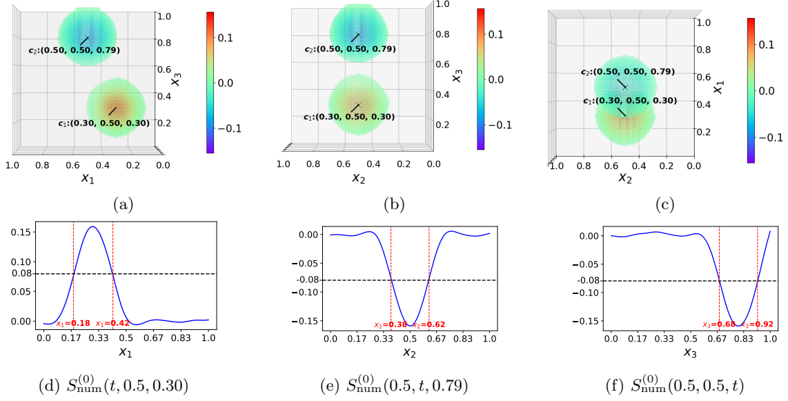
Figure 14: Example 4.7: Three-dimensional C^0 source: (a),(b),(c) show the \mathcal{Q} = \mathcal{Q}_{\text{grad}} with t_{\text{grad}} = 1/3 from different perspectives. The symbol "x" represents the center \hat{c}_1 = (0.30, 0.50, 0.30) , \hat{c}_2 = (0.50, 0.50, 0.79) , and r_1 = 0.2006 , r_2 = 0.2003 detected by Algorithm 3. (d),(e),(f) show the numerical solution g_i(t) for the slice S_{\text{num}}^{(0)} (blue solid line). The vertical black and horizontal red lines indicate the I_{\text{half}} and the corresponding position, respectively.
