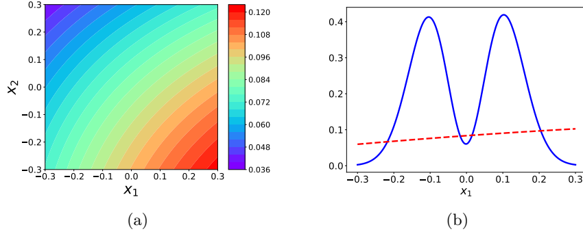
Figure 4: Example 4.2: Mountain shape source function: (a). PINN solution with u_{\text{NN}} : [2, 50, 50, 2] and S_{\text{NN}} : [2, 50, 50, 1]. (b). The true solution (—) and PINN solution (---) at (x_1, 0) .
