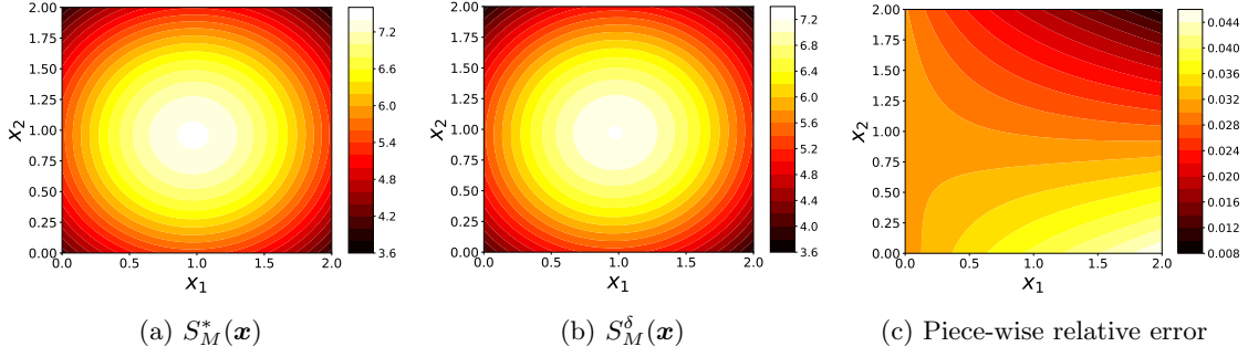
Figure 3: Example 4.1: Prior parameters: IRFM results with \eta_M = 1 , \nu = 1 , \delta = 5\% , \delta_{\text{all}} = 3.1 \times 10^{-2} , M_0 = 3200 , N_s = 15 , yield 3.01% E_{l^2}(S) .
