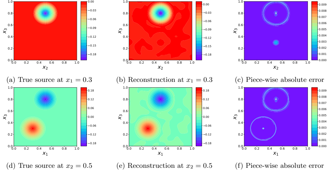
Figure 15: Example 4.7: Three-dimensional C^0 source: MA-RFM results with \delta = 5\% , M_0 = 3600 , M_{\alpha, \text{ReLU}} = M_{\alpha, \text{exp}} = 900 , \lambda_{\text{reg}}^2 = 1 \times 10^{-3} yield 1.35% E_{l^2}(S) .
