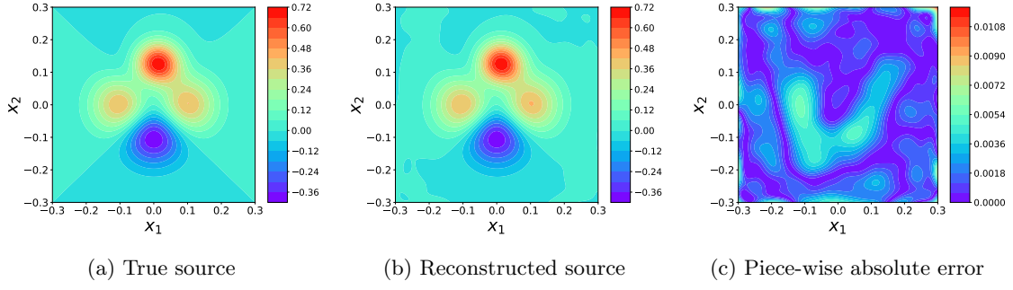
Figure 5: Example 4.2: Mountain shape source function: IA-RFM results with \delta = 10\% , M_0 = 3200 , N_s = 50 , N_\rho = 100 , \lambda_{\text{reg}}^2 = 1 \times 10^{-2} yield 1.38\% E_{l^2}(S) .
