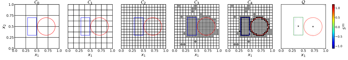
Figure 10: Example 4.5: One rectangle and one circle: grid division diagram for IA-RFM with \delta = 5\% , M_0 = 2400 , \text{Tanh} , R_m = 2 . The last one shows the \mathcal{Q} = \mathcal{Q}_{\text{abs}} \cap \mathcal{Q}_{\text{grad}} , with t_{\text{grad}} = t_{\text{abs}} = 1/3 . The red and green dashed lines indicate the detected boundary, while the “ \times ” symbols denote the detected center obtained by Algorithm 3.
