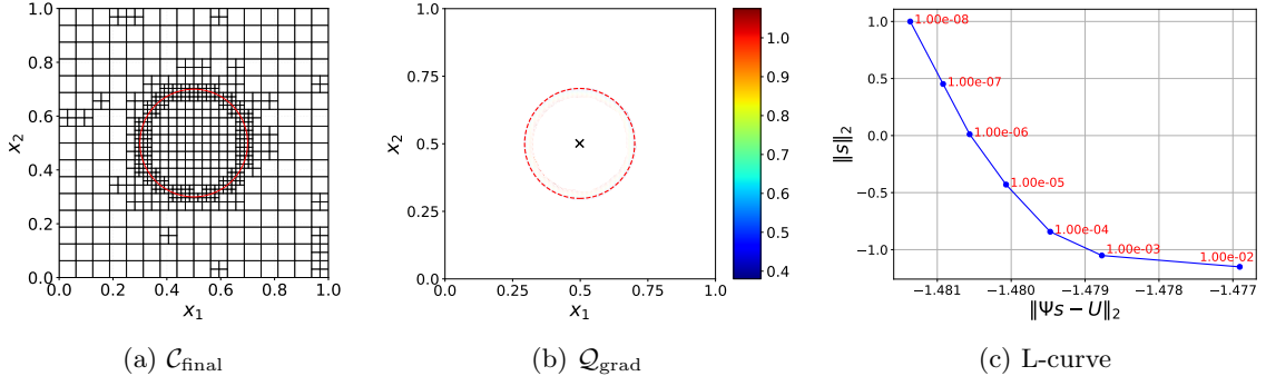
Figure 6: Example 4.3: Discontinuous source: (a) shows the \mathcal{C}_{\text{final}} with IA-RFM, and the red line represents the true interface. (b) displays the \mathcal{Q}_{\text{grad}} with t_{\text{grad}} = 1/3 . The red dashed lines indicate the detected boundary, while the “x” symbols denote the detected center obtained by Algorithm 3. (c) records the L-curve \log_{10}(\|\Psi \cdot \mathbf{s} - U\|_2) - \log_{10}(\|\mathbf{s}\|_2) with different \lambda_{\text{reg}}^2 .
