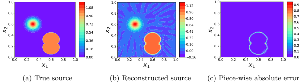
Figure 13: Example 4.6: Complex geometry: MA-RFM results with \delta = 5\% , M_0 = 1600 , M_1 = 1600 , M_2 = 1783 , \lambda_{\text{reg}}^2 = 1 \times 10^{-2} yield 12.67\% E_{l^2}(S) .
