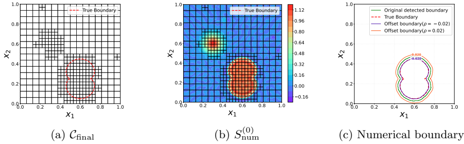
Figure 12: Example 4.6: Complex geometry: (a)-(b) Final adaptive mesh ( \mathcal{C}_{\text{final}} ) and reconstruction obtained via IA-RFM, yielding a relative error of E_{l^2}(S) = 19.74\% with n_{\text{integral}} = 4113 . (c) Numerical boundary reconstruction. The true boundary (red dashed) is compared with the nominal boundary extracted from \mathcal{Q}_{\text{grad}} with t_{\text{grad}} = 1/3 (green solid). The orange and purple contours represent the perturbed numerical level sets ( \rho = \pm 0.02 ).
