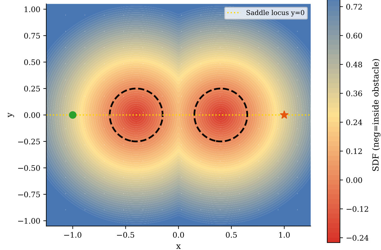
Obstacle Signed Distance Field + Gradient Flow
