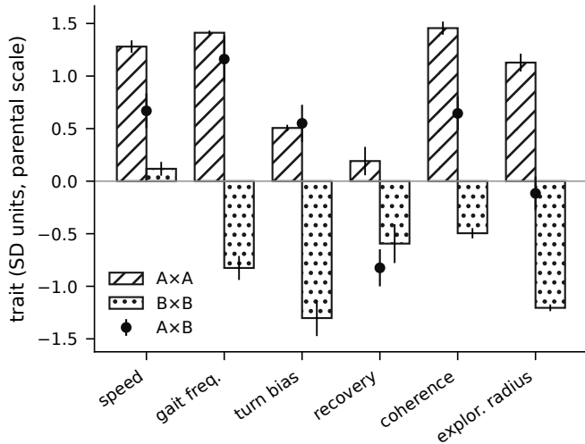
Clone lines vs biparental offspring
