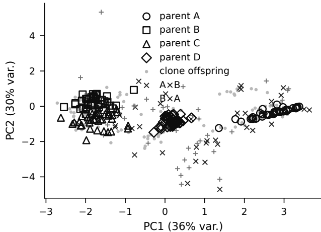
Phenotype space (standardised traits)
