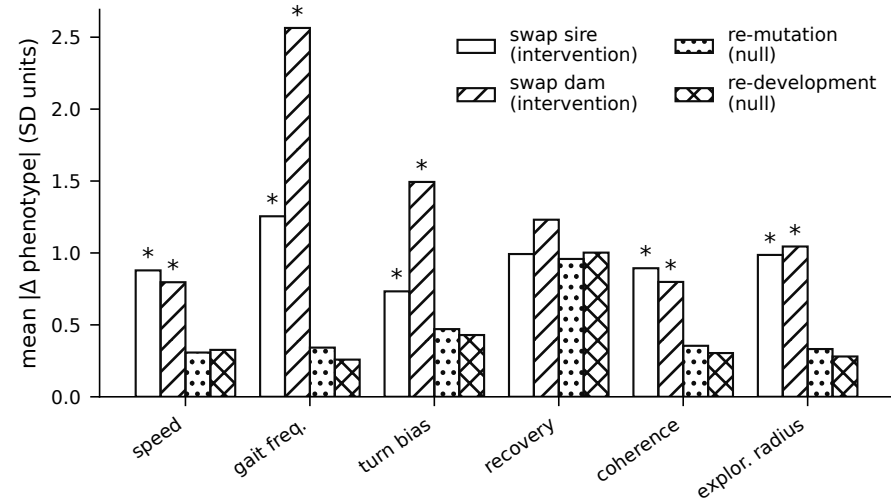
Germline swap on matched backgrounds (base AxB, n=60)
