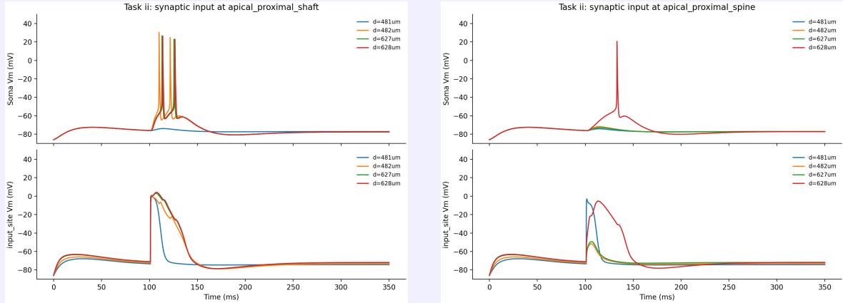
Figure 10: Voltage responses for a single synapse ( w = 0.6 ) placed at varying distances along the apical shaft (left) and spine (right).
