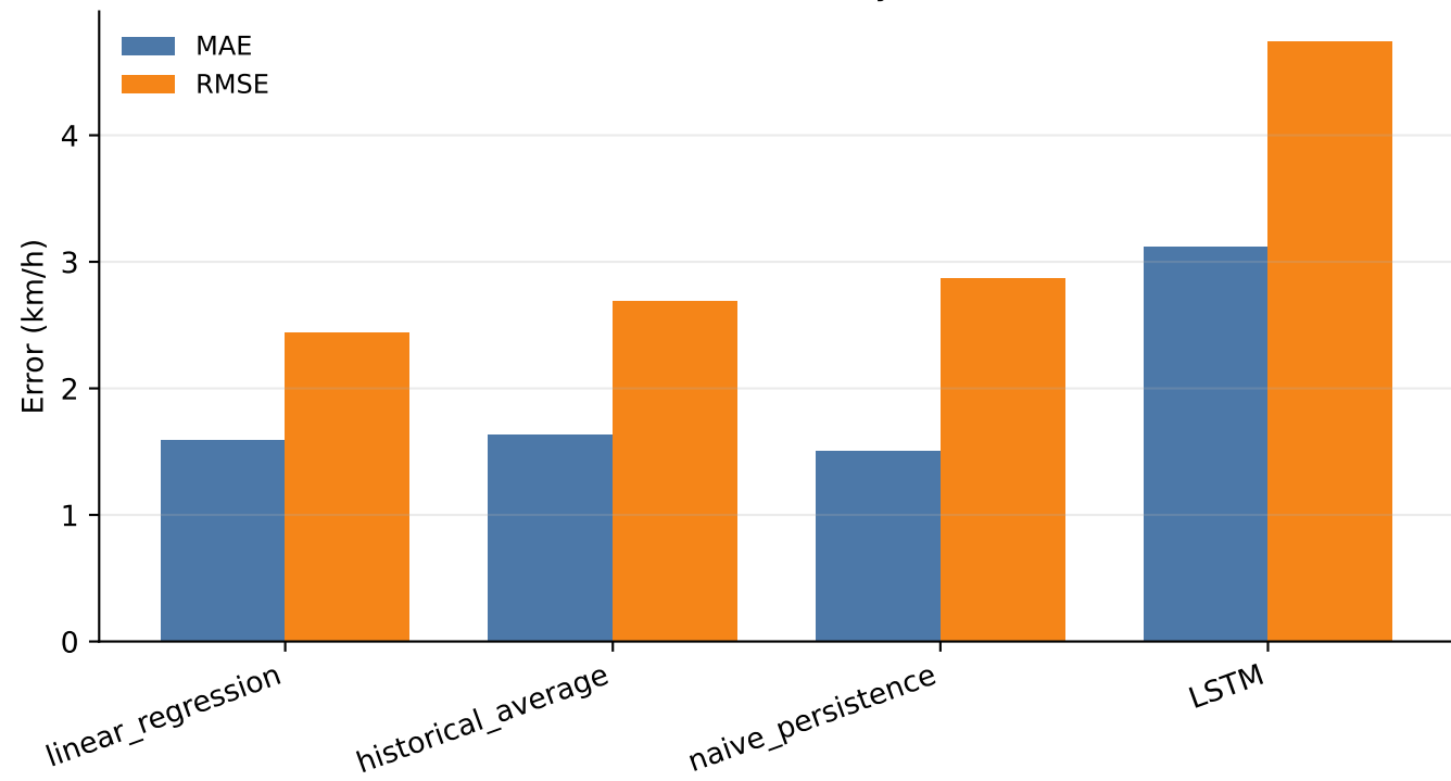
Overall Test Error by Model
