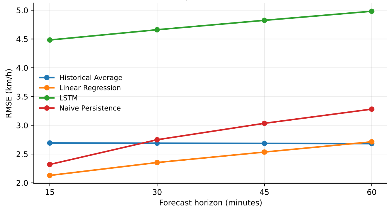
RMSE by Forecast Horizon
