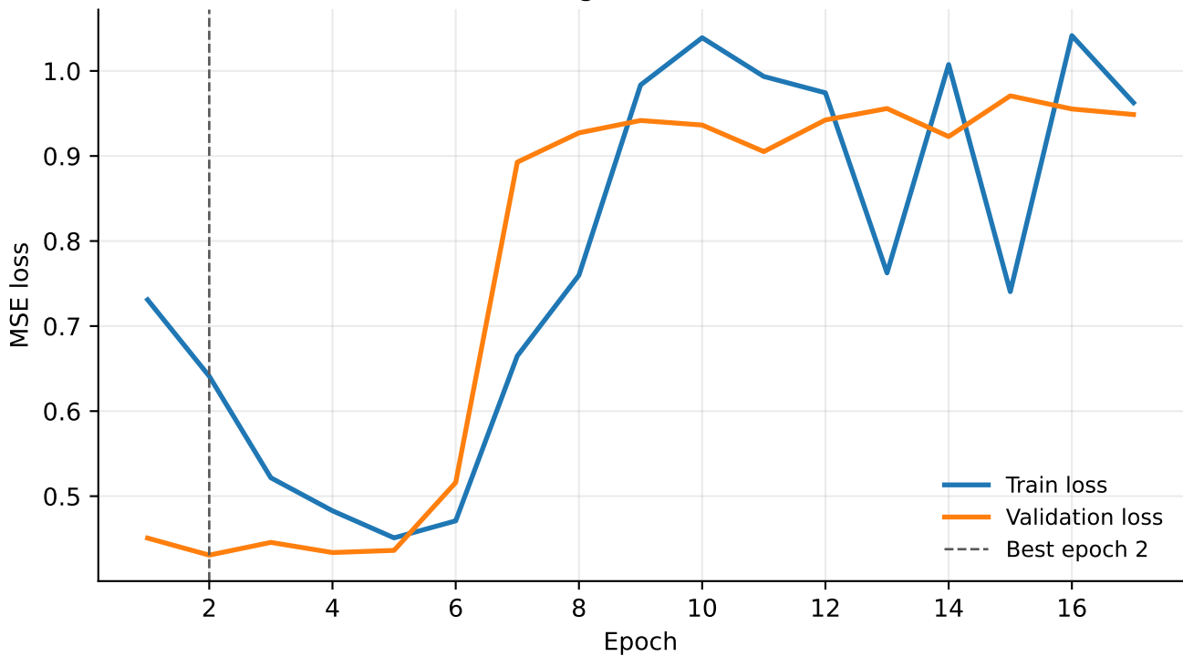
LSTM Training and Validation Loss
