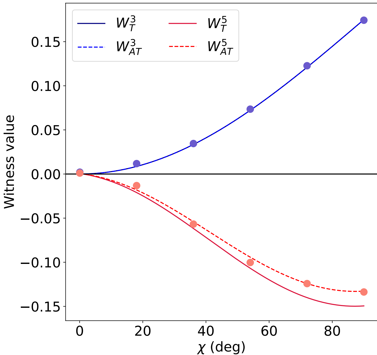
Entangled State Witnessed by 1st W5 Triplet (2025)
