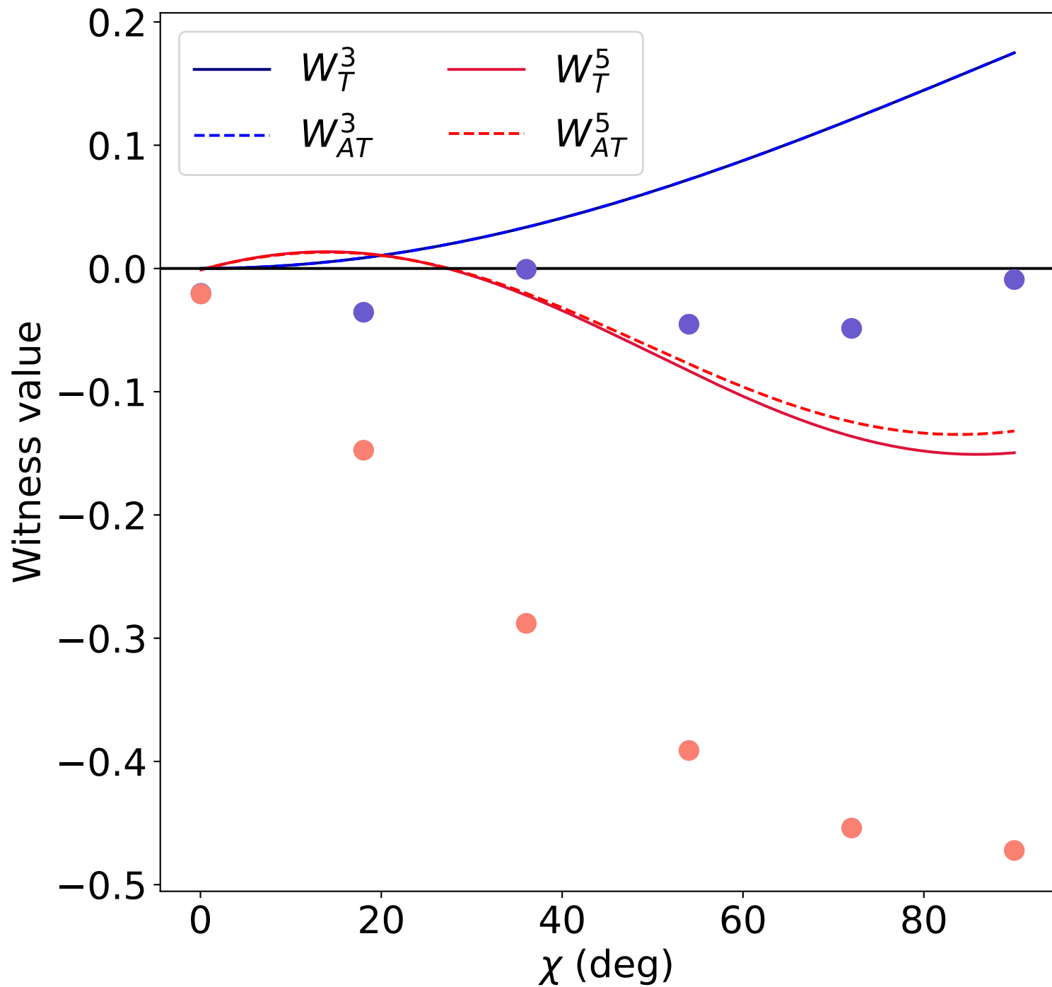
Entangled State Witnessed by 2nd W5 Triplet (2025)
