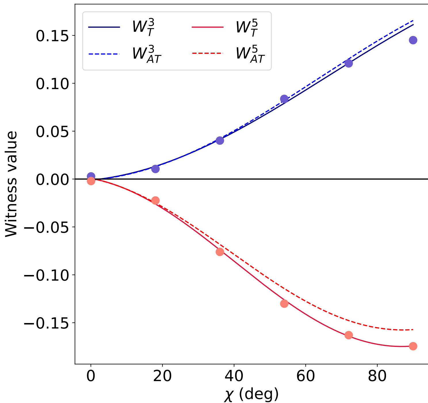
Entangled State Witnessed by 3rd W5 Triplet (2025)
