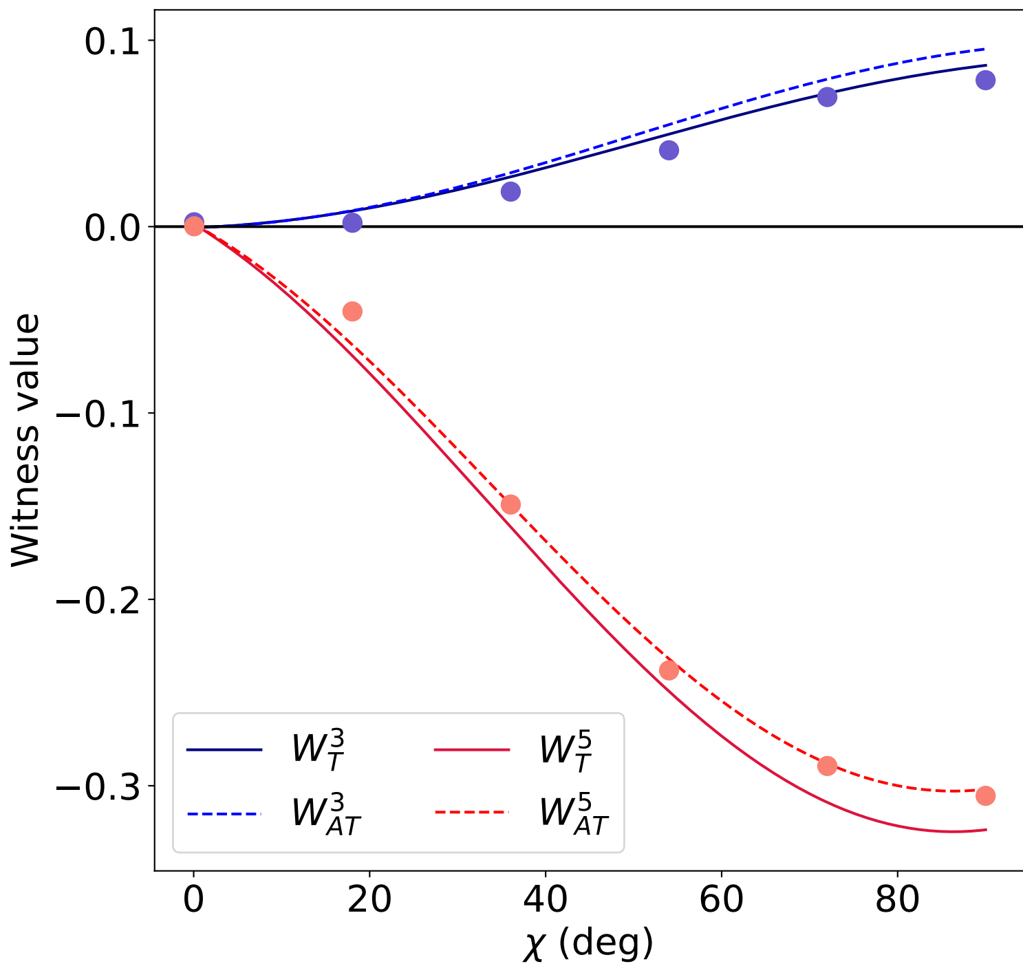
Entangled State Witnessed by 2nd W5 Triplet (2025)
