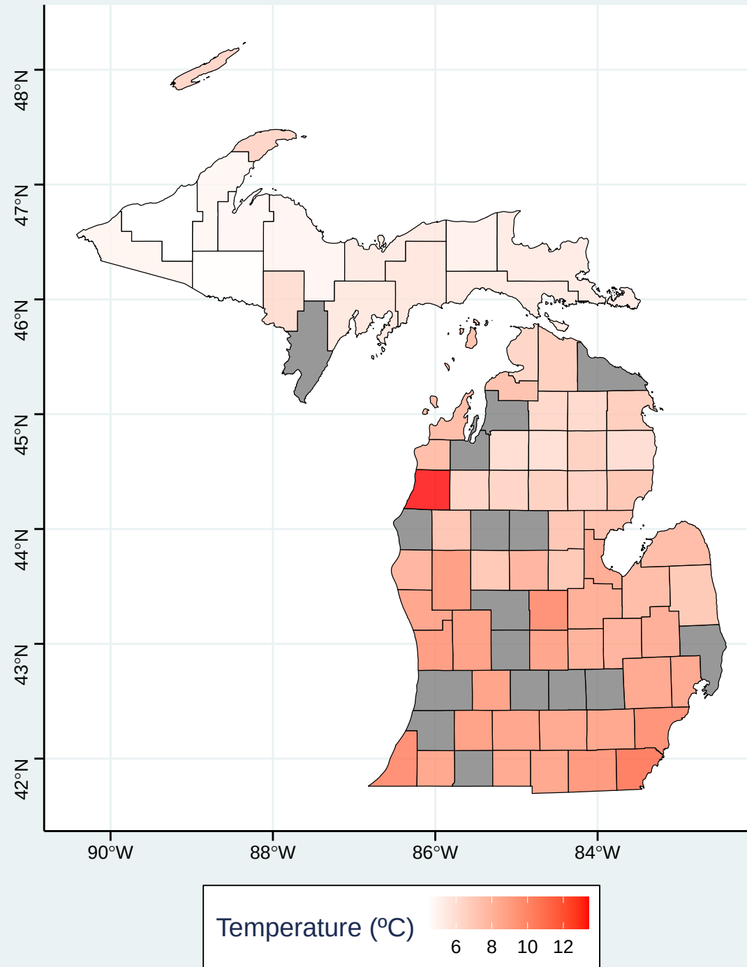
Michigan County by 2025 Average Air Temperature Map
