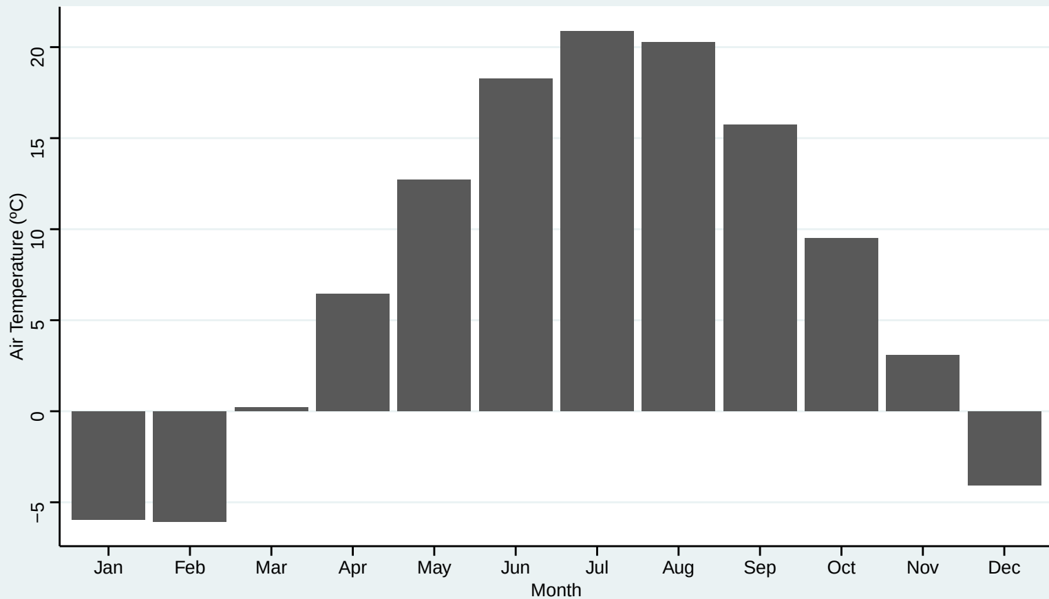
Michigan Average Air Temperature by Calendar Month
