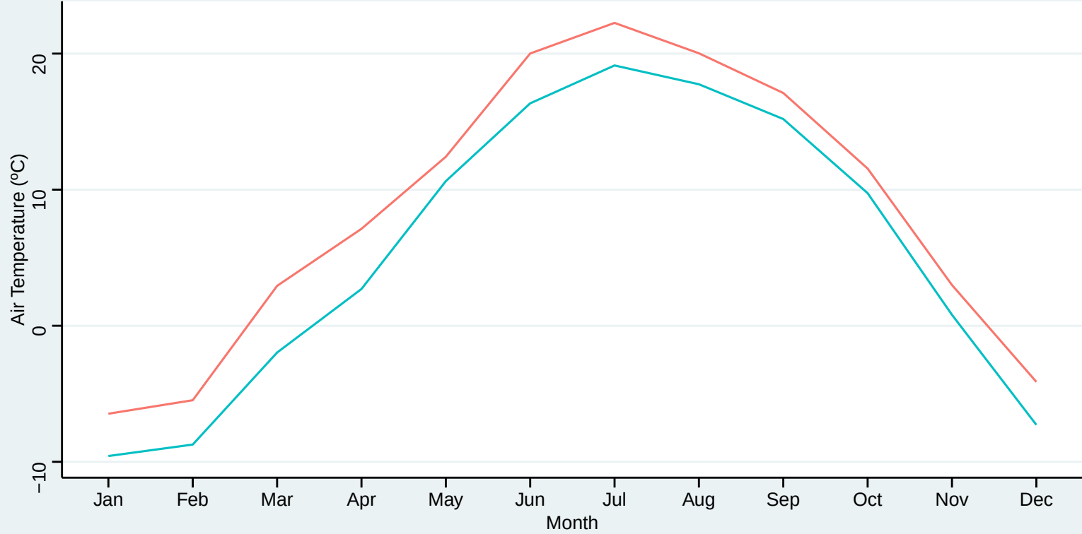
Average 2025 Air Temperature by Month and Peninsula
