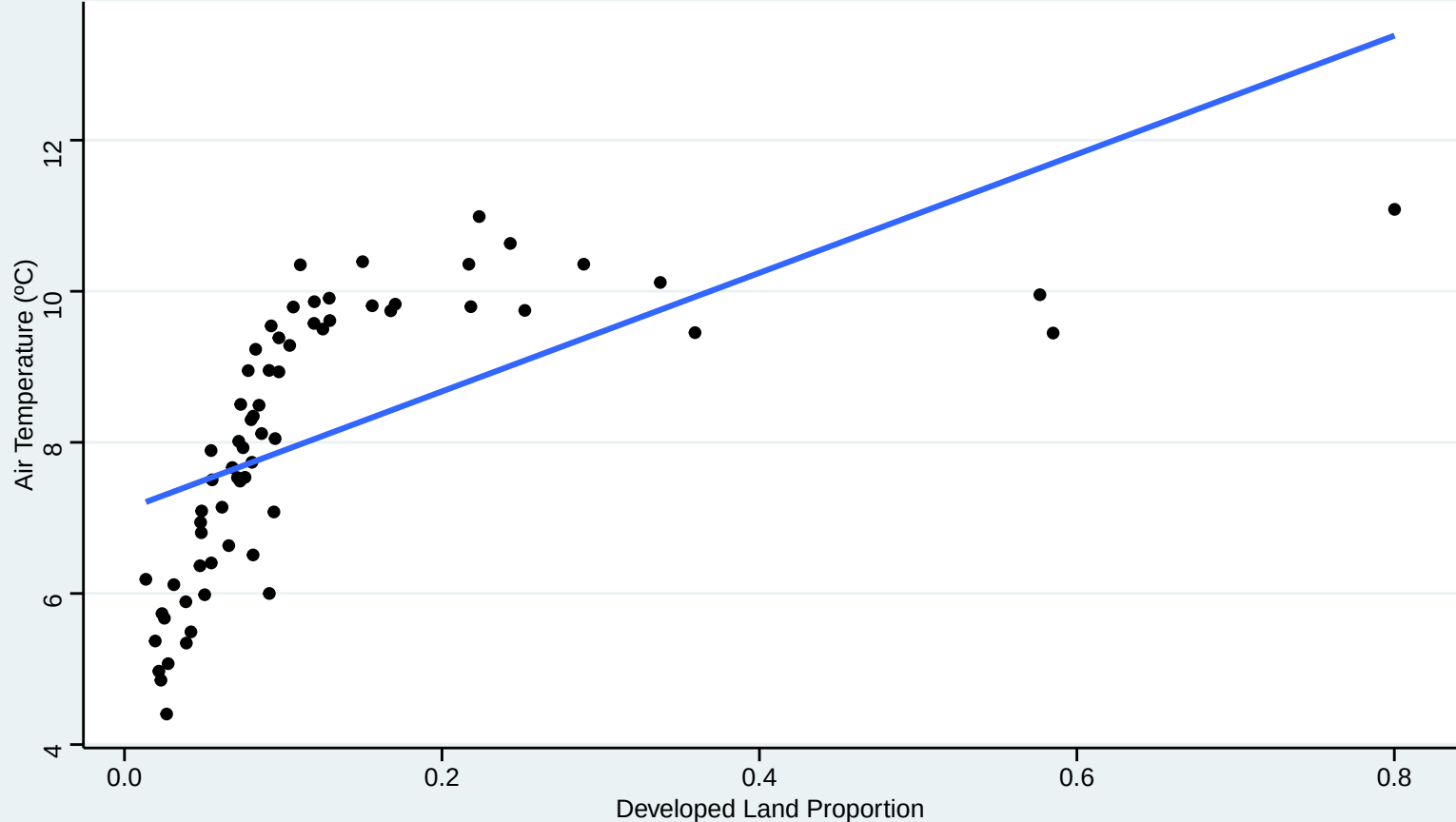
Average 2020 Air Temperature by Michigan County Developed Land Proportion
